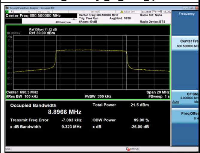
FDD71_MidRange_10_680.5_Q16
