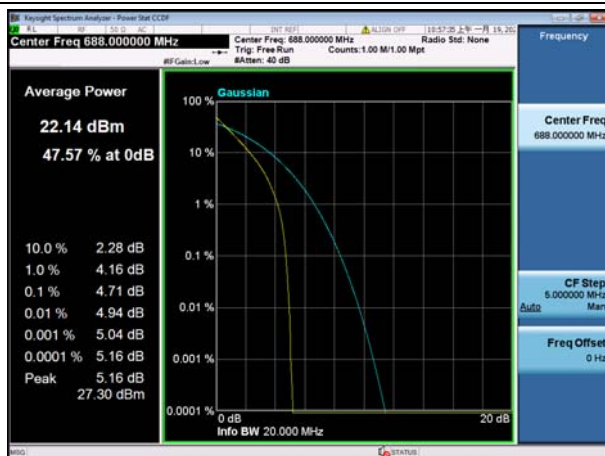
FDD71_HighRange_20MHz_688_OneRB _high_Q16
