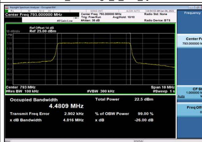
FDD14_MidRange_5_793_QPSK
