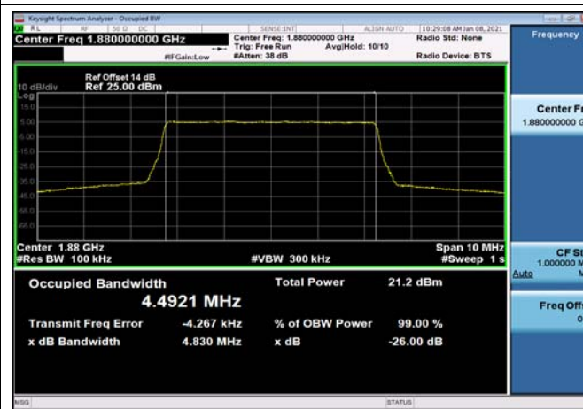
FDD02_MidRange_10_1880_QPSK
