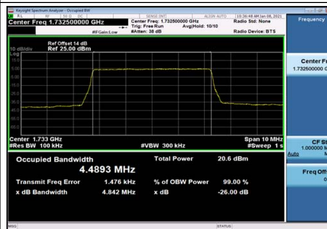
FDD04_MidRange_10_1732.5_QPSK
