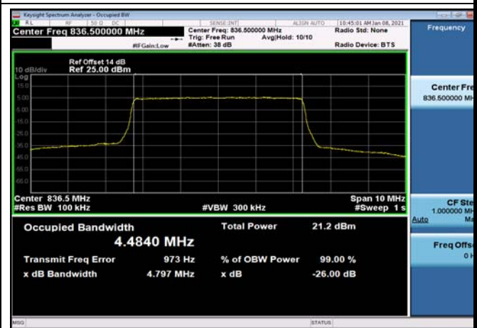
FDD05_MidRange_10_836.5_Q16
