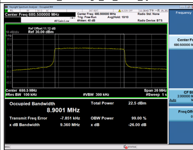
FDD71_MidRange_10_680.5_QPSK
