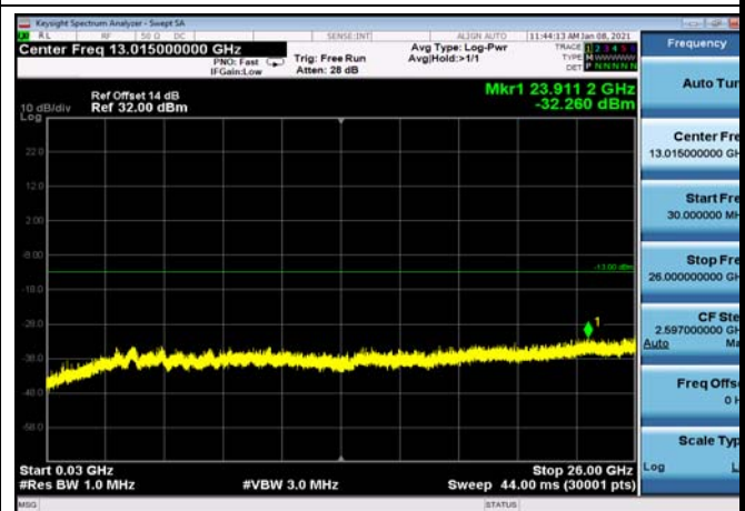
FDD66_LowRange_5MHz_30MHz~26GHz
