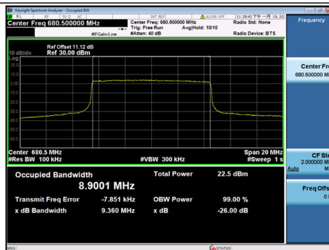
FDD71_MidRange_10_680.5_QPSK
