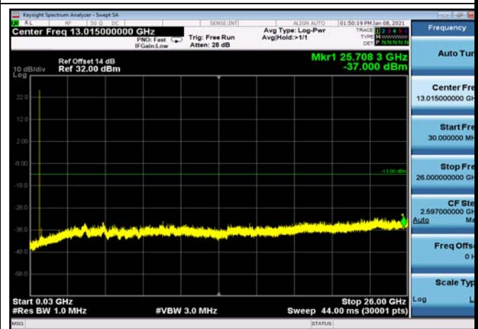
FDD12_MidRange_10MHz_30MHz~26GHz
