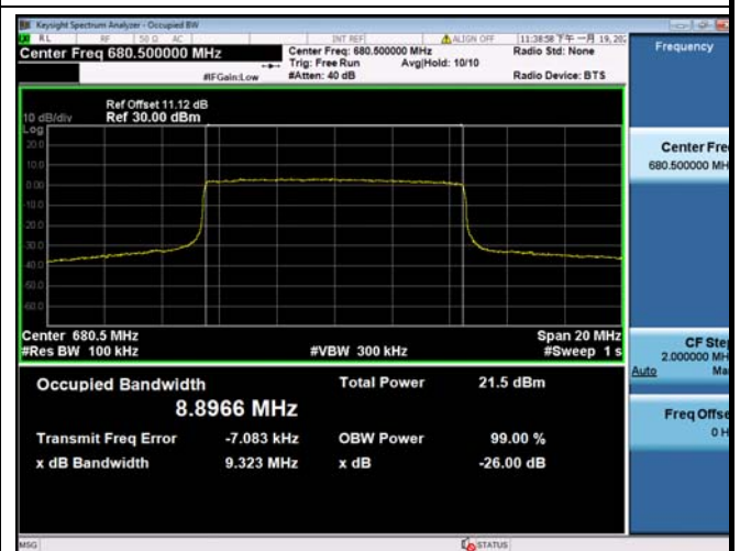
FDD71_MidRange_10_680.5_Q16
