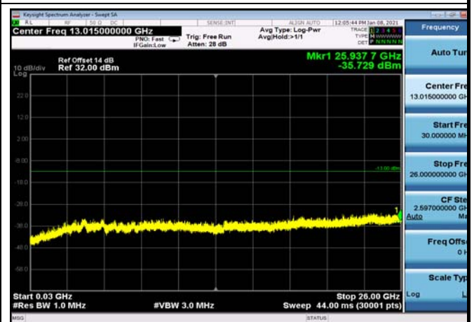
FDD66_HighRange_20MHz_30MHz~26GHz
