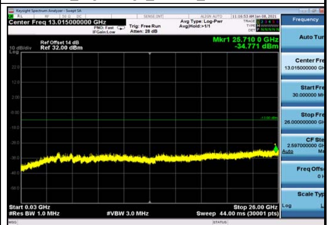
FDD66_HighRange_5MHz_30MHz~26GHz
