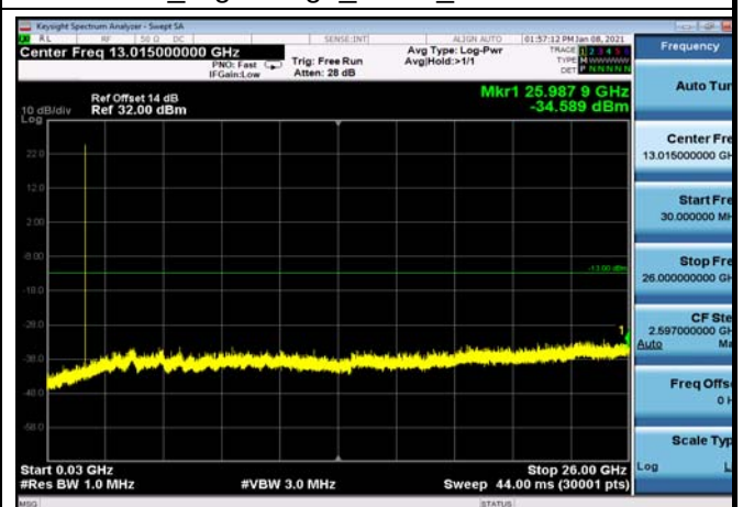
FDD66_HighRange_5MHz_30MHz~26GHz
