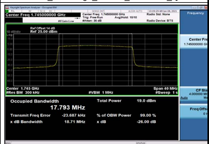
FDD66_MidRange_20MHz_1745MHz_Q16
