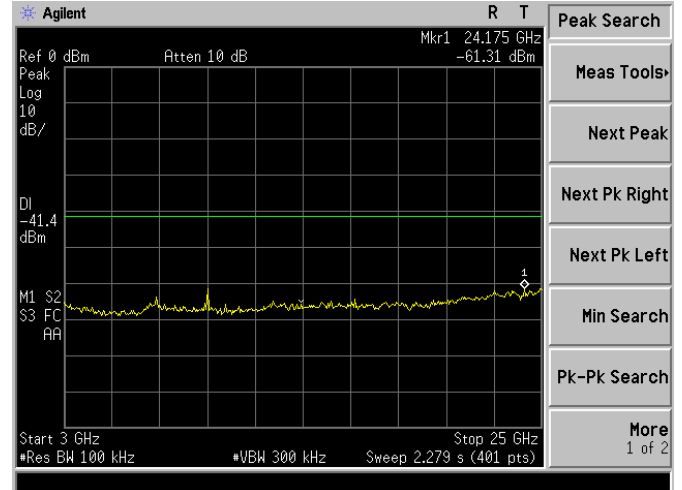
Low Channel 2405MHz
