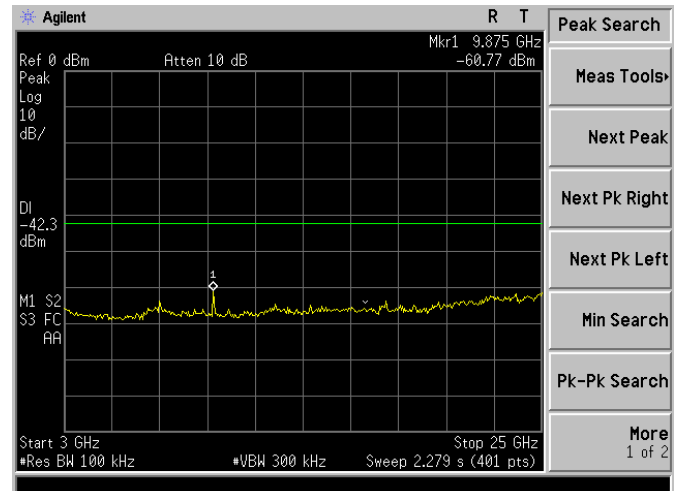
High Channel 2470MHz
