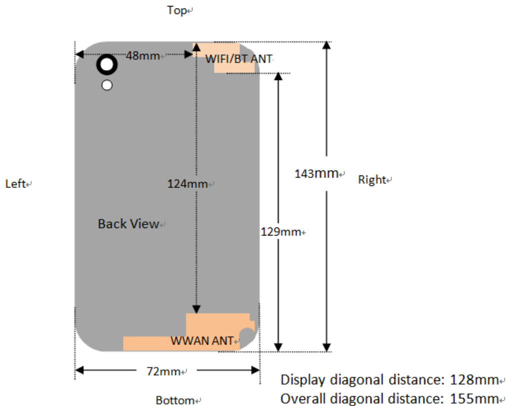
Fig.14.1 EUT Antenna Locations
