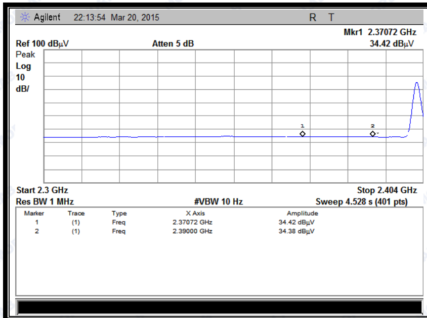
(Plot A2:Channel = 0 AVERAGE @ GFSK)
