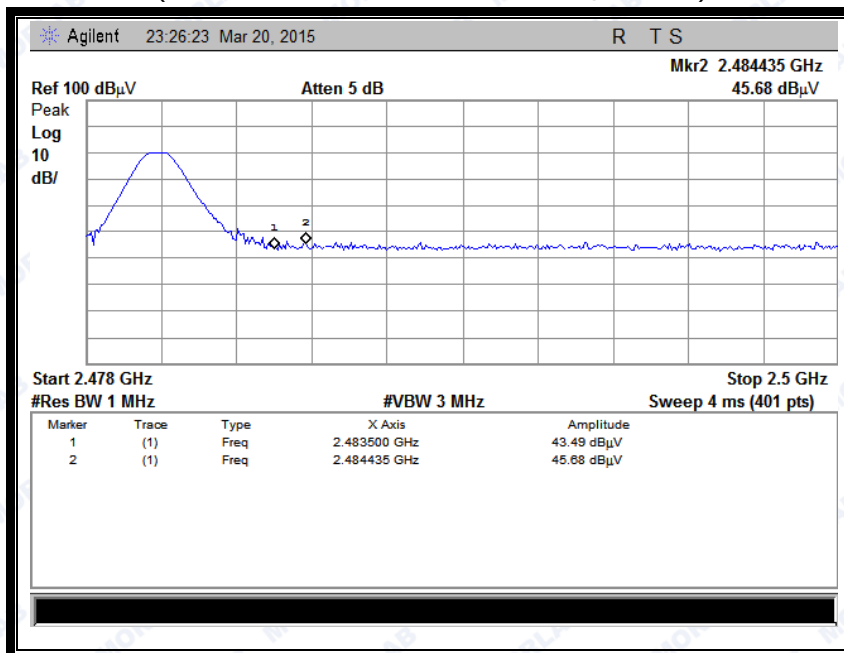
(Plot B1:Channel = 78 PEAK @ GFSK)
