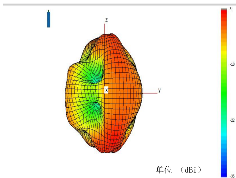
Channel (MHz) 2440
