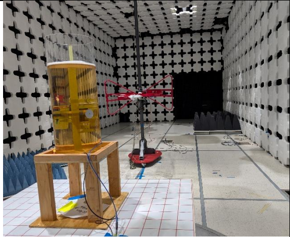
Radiated Spurious Emission-Below 1GHz-Back (Tined Lead)
