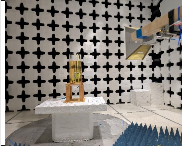
Radiated Spurious Emission-Above 1GHz-Front (2XPNE Lead)
