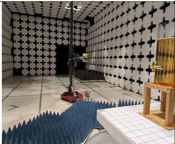
Radiated Spurious Emission-Above 1GHz-Back (Tined lead)
