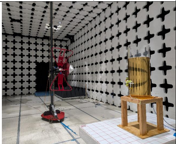
Radiated Spurious Emission-Below 1GHz-Back (2XPNE Lead)
