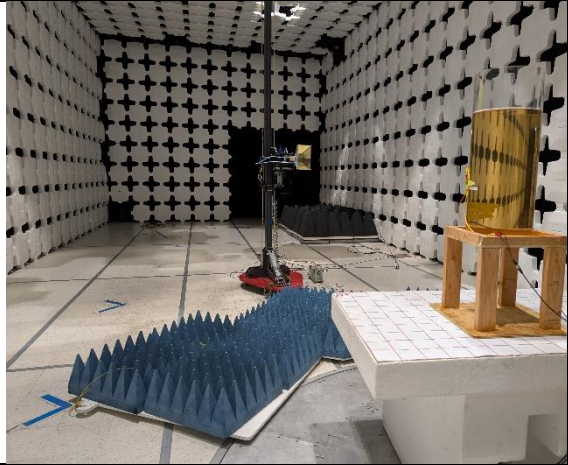
Radiated Spurious Emission-Above 1GHz-Back ( 2XPNE Lead )
