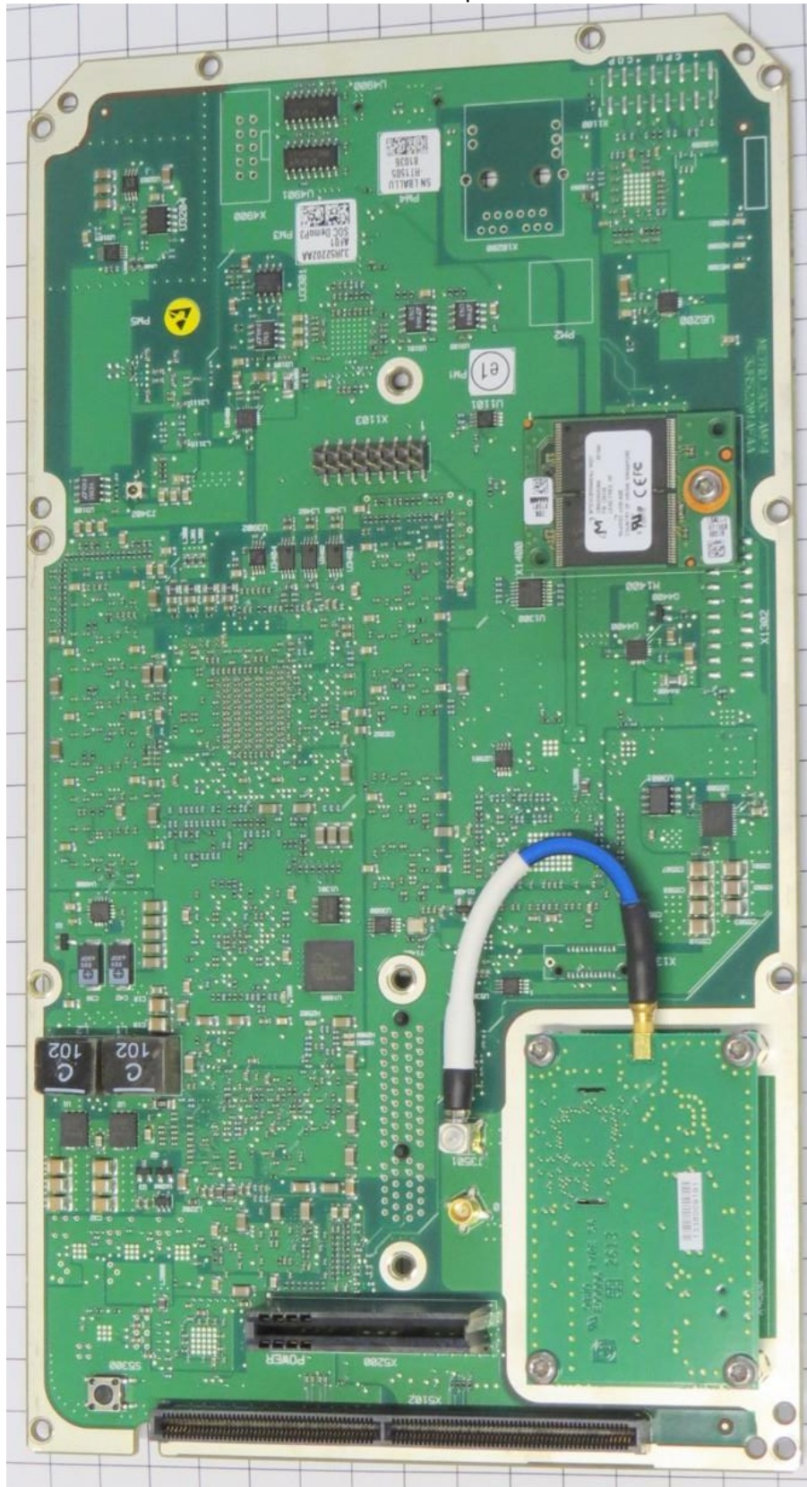
Modem board top view
