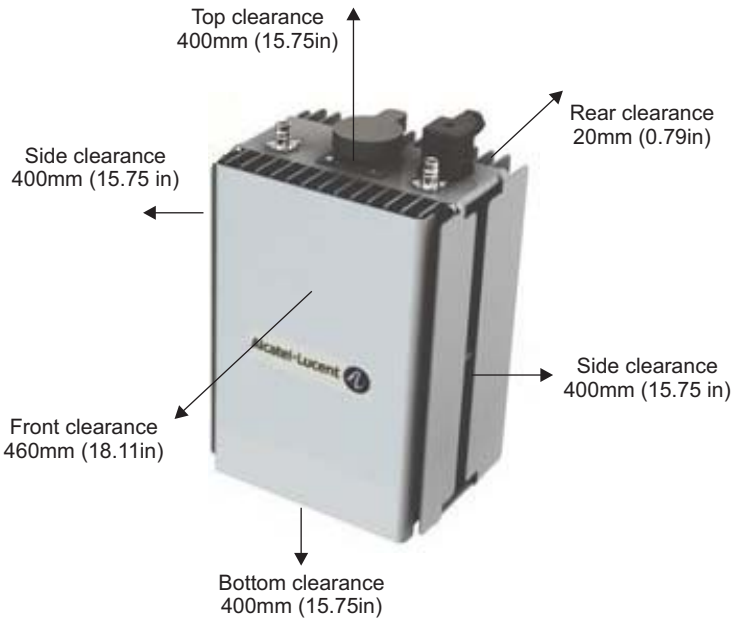
Figure 3-2 9764 CMCO B41 2x6W installation clearances
