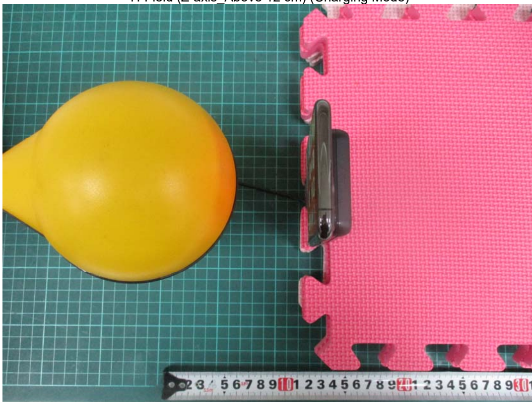
H-Field (Z-axis_Above 12 cm) (Charging Mode)
