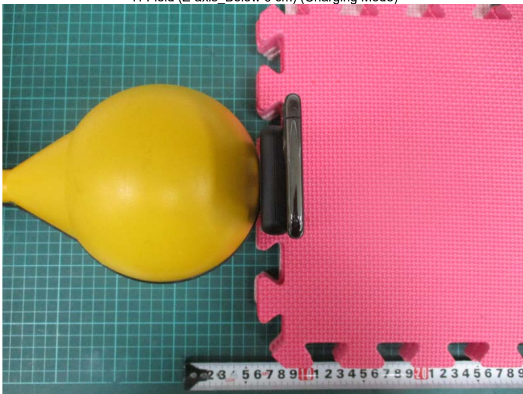
H-Field (Z-axis_Below 6 cm) (Charging Mode)
