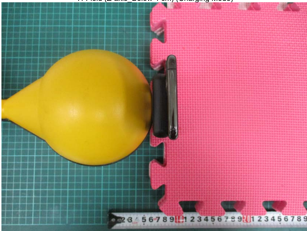
H-Field (Z-axis_Below 4 cm) (Charging Mode)
