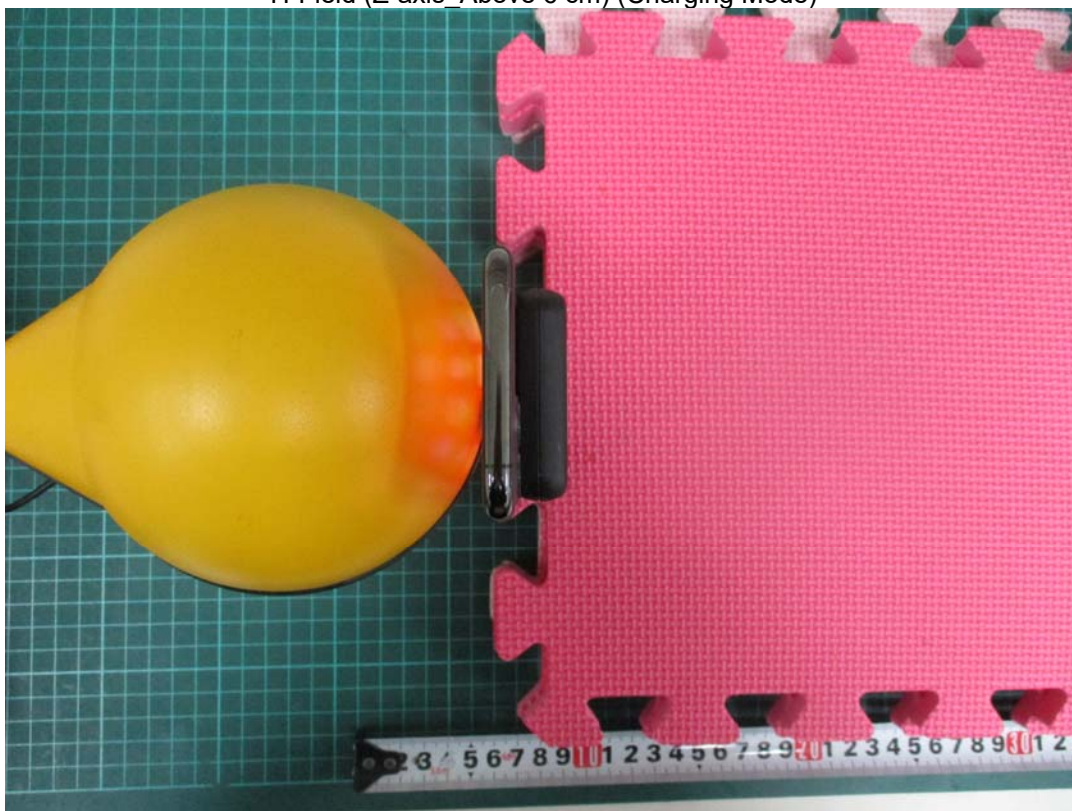
H-Field (Z-axis_Above 6 cm) (Charging Mode)
