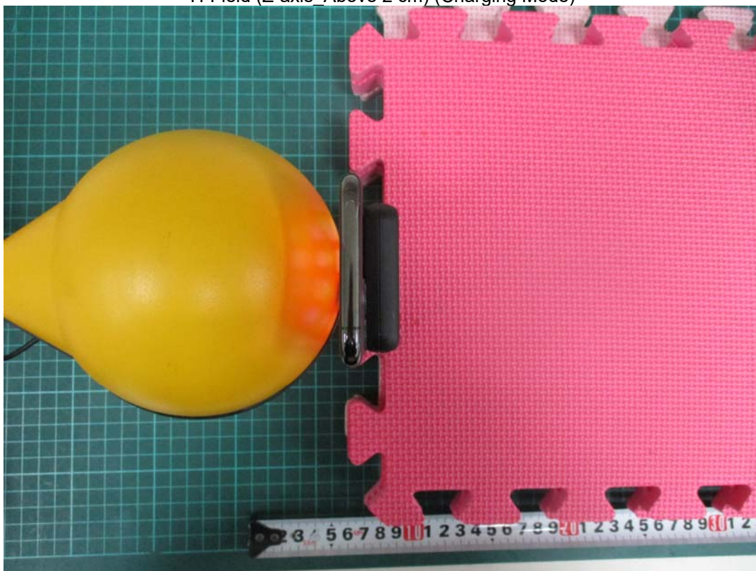
H-Field (Z-axis_Above 2 cm) (Charging Mode)
