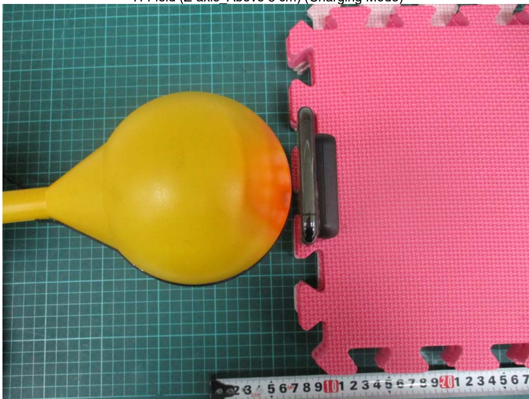
H-Field (Z-axis_Above 8 cm) (Charging Mode)
