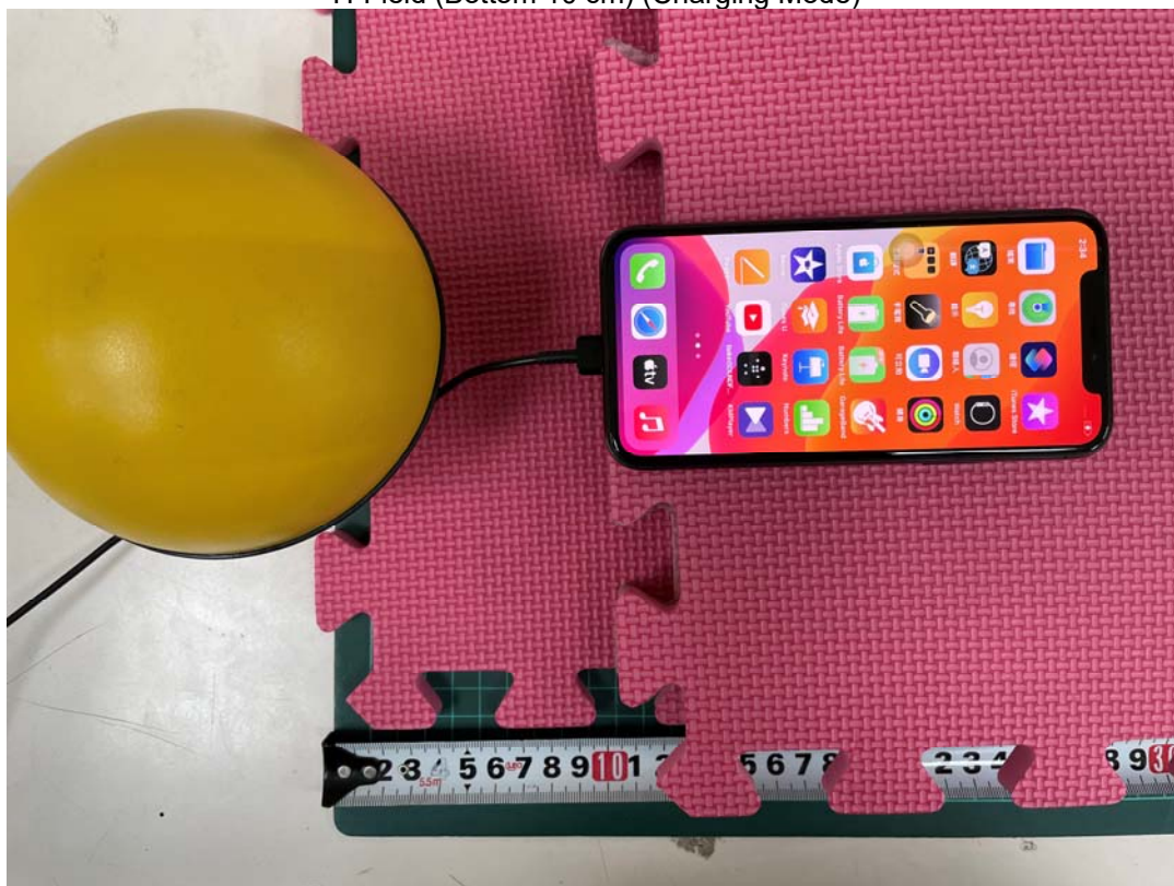
H-Field (Bottom 10 cm) (Charging Mode)
