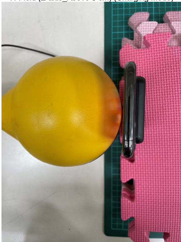
H-Field (Z-axis_Above 0 cm) (Charging Mode)
