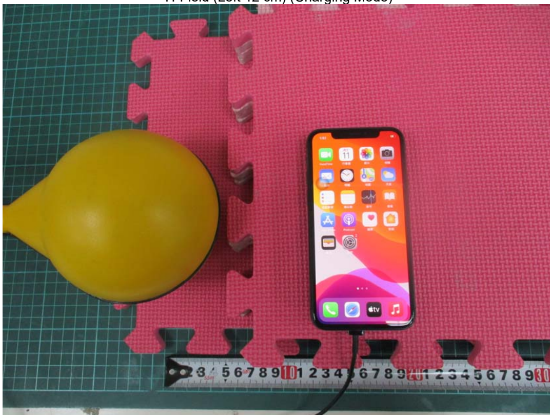
H-Field (Left 12 cm) (Charging Mode)
