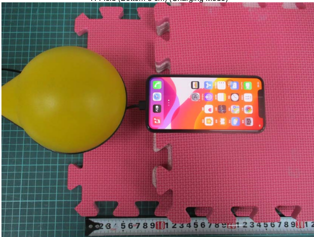
H-Field (Bottom 8 cm) (Charging Mode)
