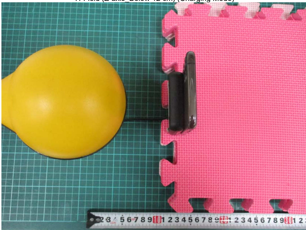
H-Field (Z-axis_Below 12 cm) (Charging Mode)
