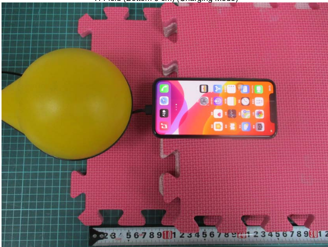
H-Field (Bottom 6 cm) (Charging Mode)
