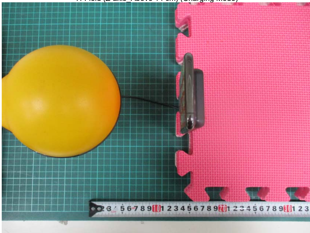
H-Field (Z-axis_Above 14 cm) (Charging Mode)
