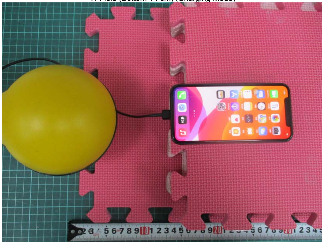
H-Field (Bottom 14 cm) (Charging Mode)
