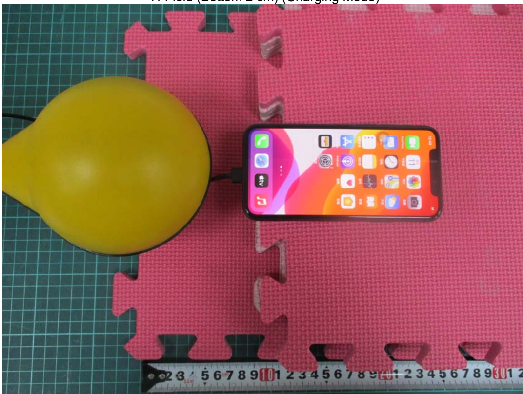
H-Field (Bottom 2 cm) (Charging Mode)
