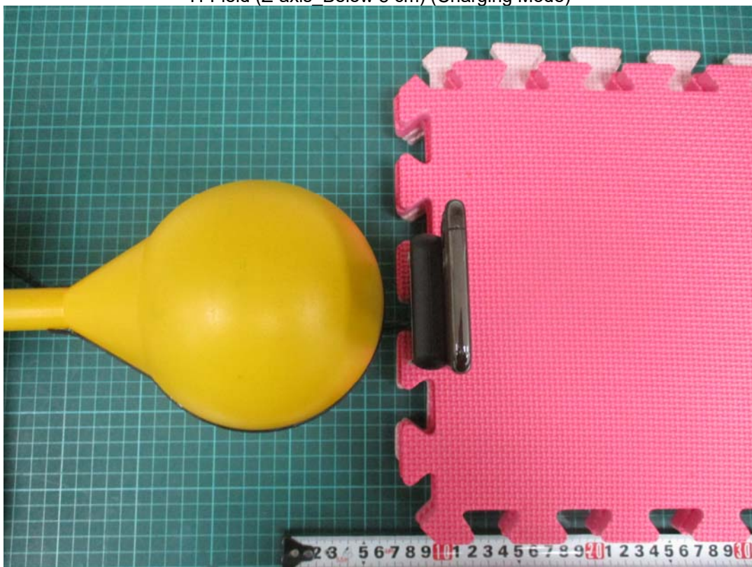
H-Field (Z-axis_Below 8 cm) (Charging Mode)
