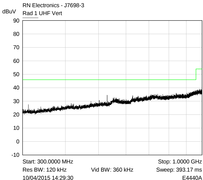
Plot of peak vertical emissions 300MHz - 1000MHz against the quasi-peak limit line.
