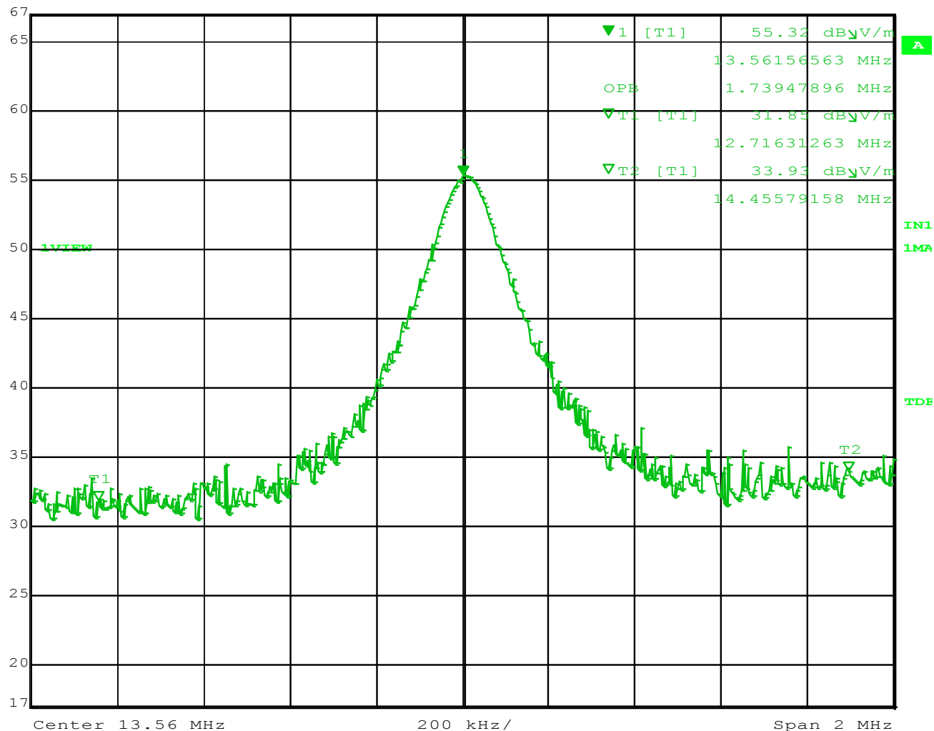
Figure 10 – 99% Bandwidth
