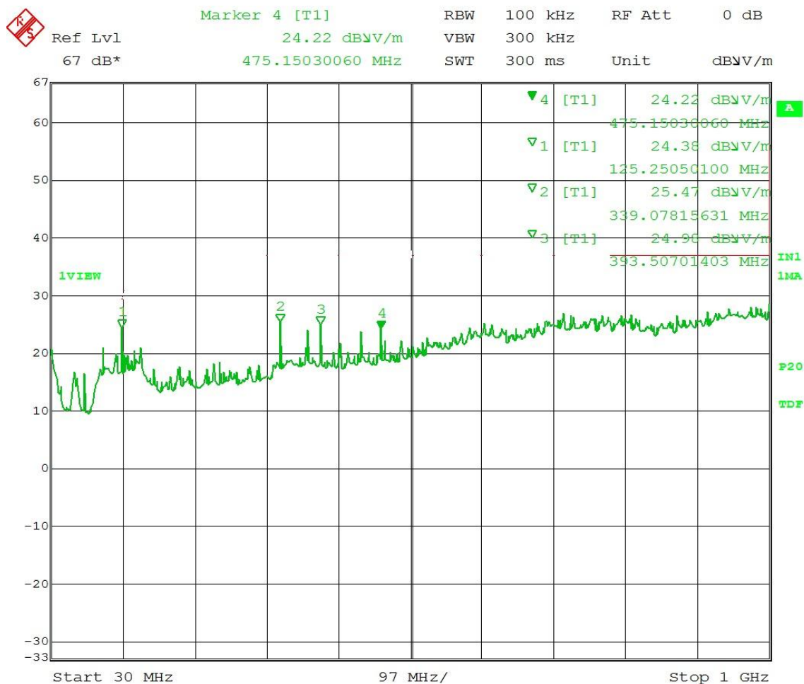
Figure 1 – Horizontal 30 – 1000 MHz
