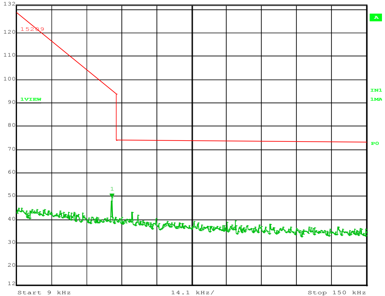
Figure 6 – Spurious Emissions (Parallel) 9 kHz to 150 kHz
