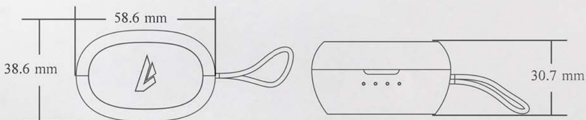
Charging box
