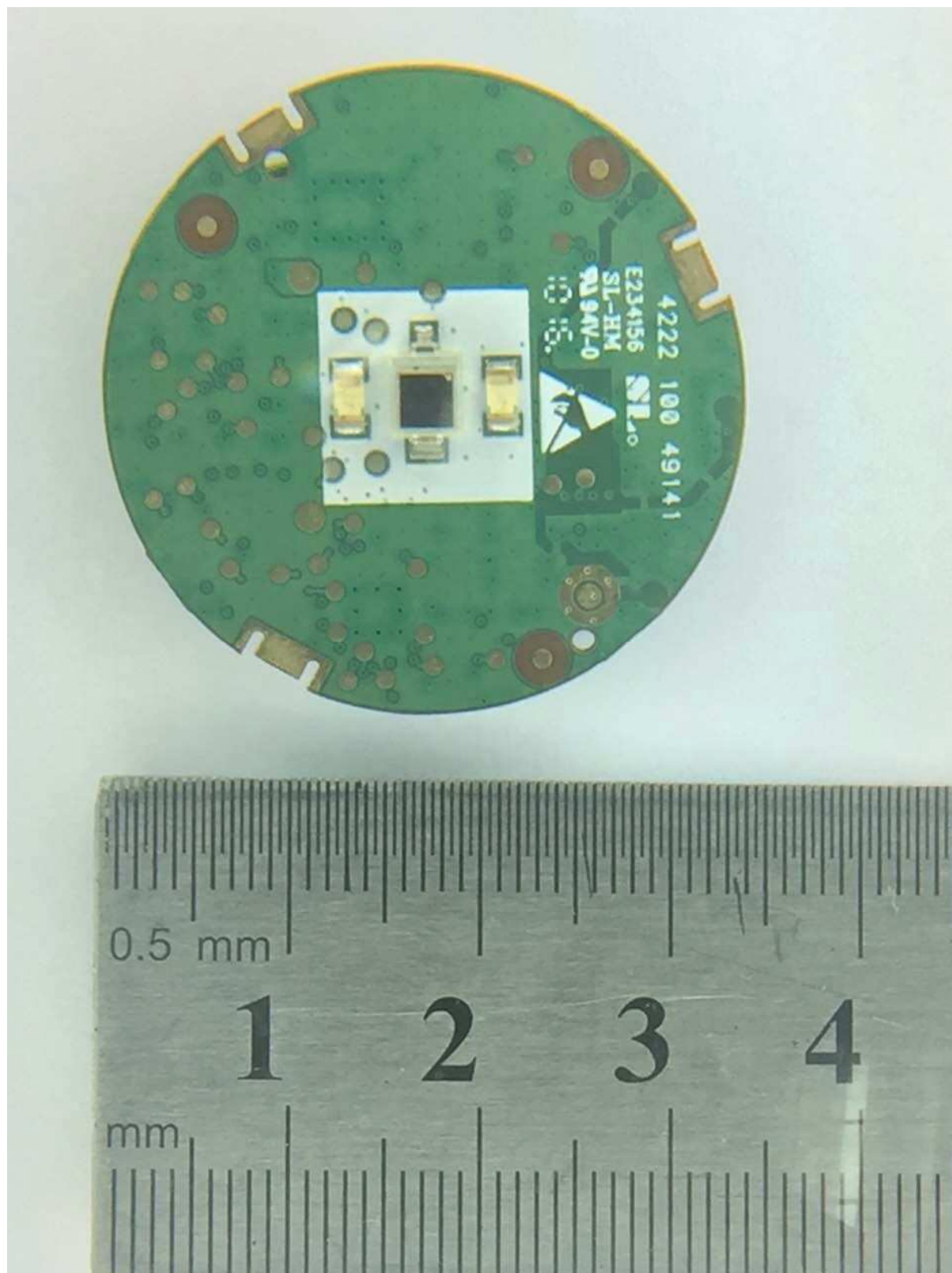
Figure 4: PCB backside view
