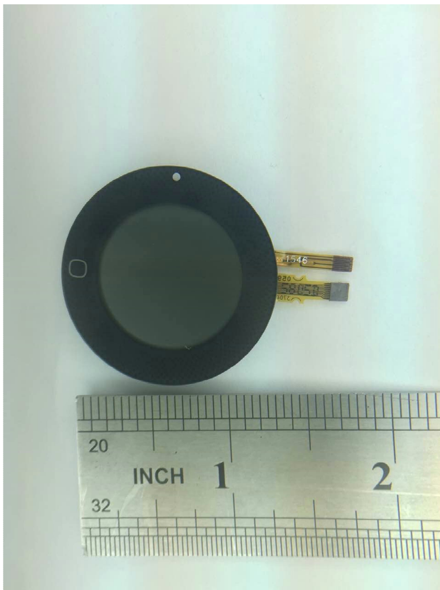
Figure 5: Display assembly, including antenna, frontside view
