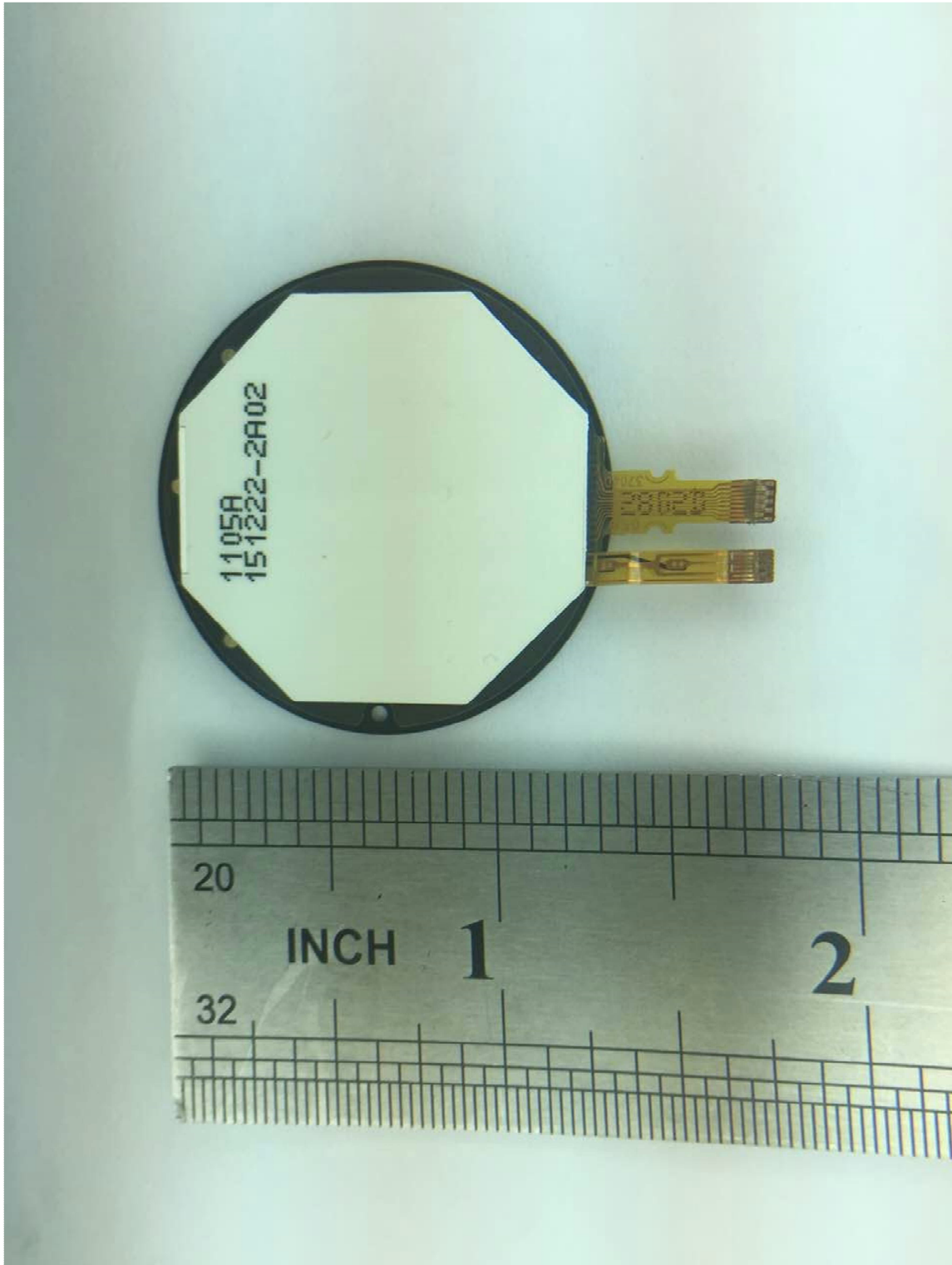
Figure 6: Display assembly, including antenna, backside view
