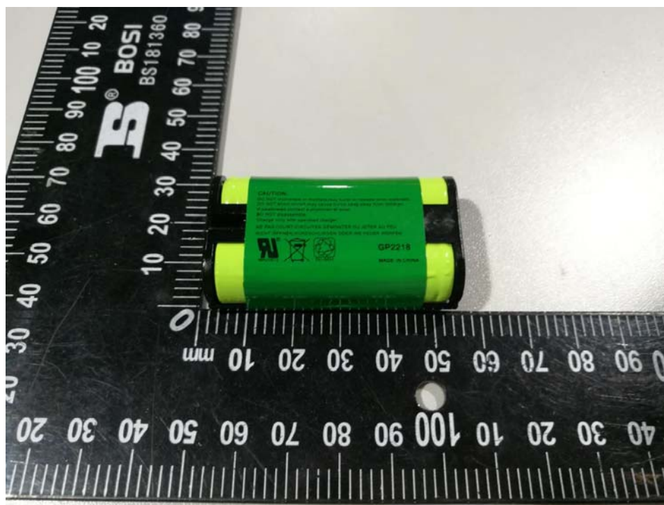
Figure 4 – 2.4VDC (1 x 2.4V 1300mAh Ni-MH rechargeable battery pack)
