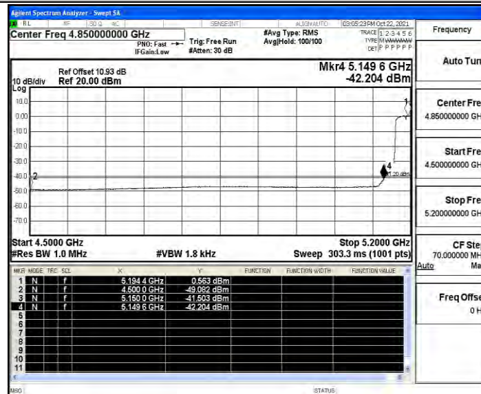
11N40SISO_Ant0_Low_5190_Peak
