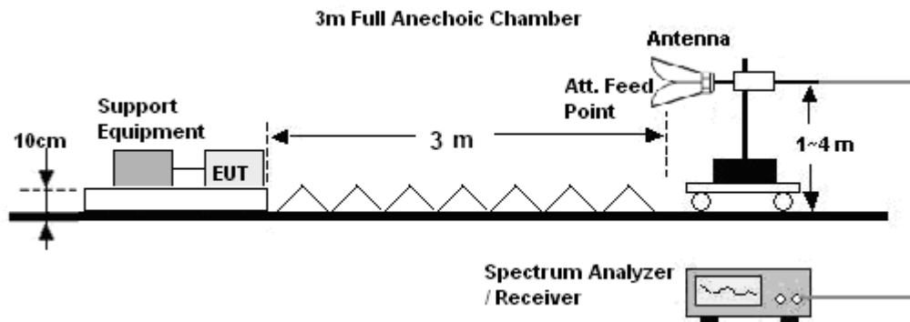
Figure 2. Above 1GHz
