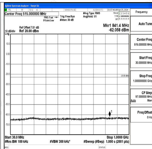
Band4_20MHz_QPSK_20050_1RB#0_30~1000_30~1000 0
