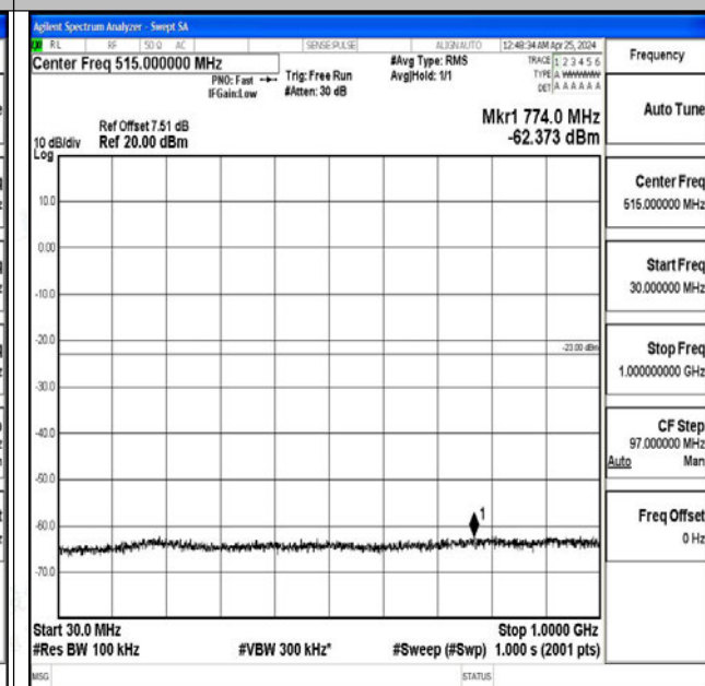
Band4_15MHz_QPSK_20325_1RB#0_30~1000_30~1000
