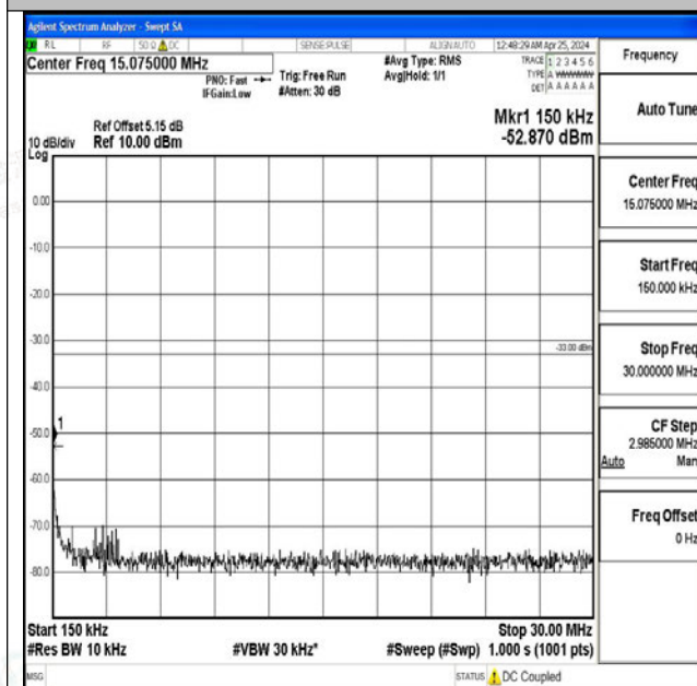
Band4_15MHz_QPSK_20325_1RB#0_0.15~30_0.15~30
