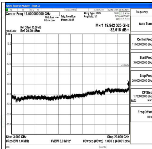
Band4_15MHz_16QAM_20175_1RB#0_3000~20000_3000~20000
