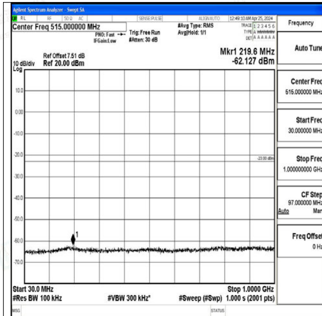
Band4_15MHz_16QAM_20325_1RB#0_30~1000_30~1000
