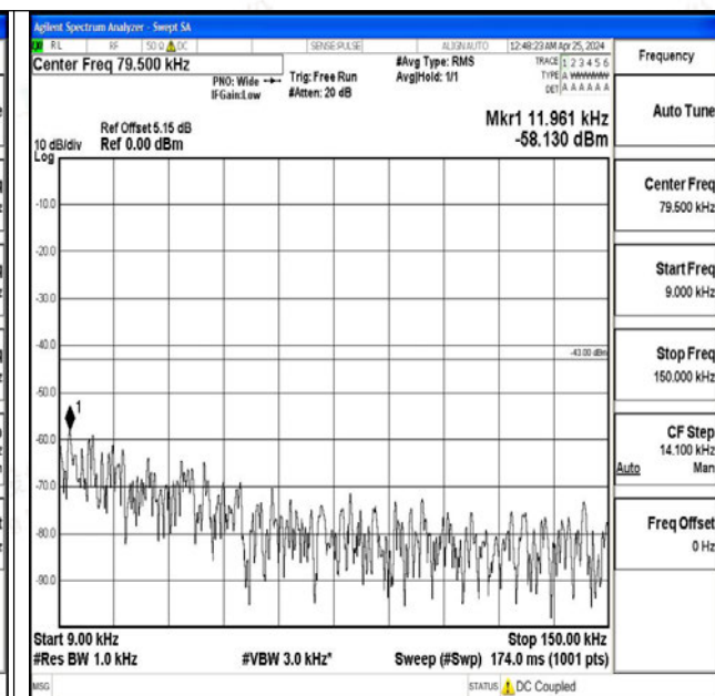
Band4_15MHz_QPSK_20325_1RB#0_0.009~0.15_0.009~0.15
