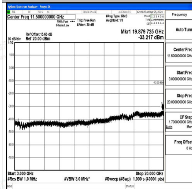
Band4_15MHz_16QAM_20325_1RB#0_3000~20000_3000~20000
