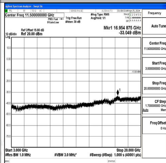
Band4_20MHz_QPSK_20050_1RB#0_3000~20000_3000 0~20000
