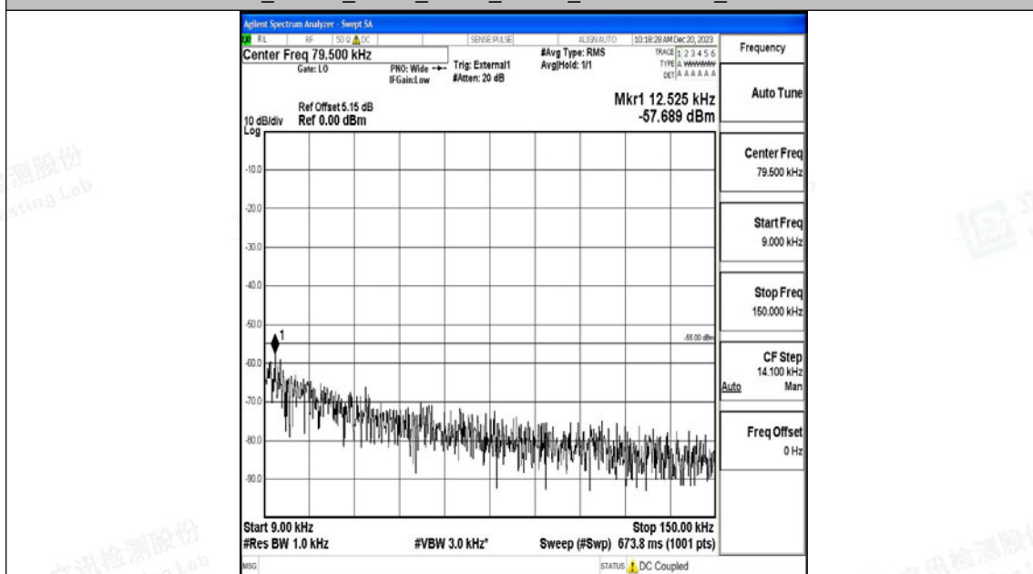
Band41_20MHz_16QAM_39750_1RB#0_0.009~0.15_0.009~0.15
