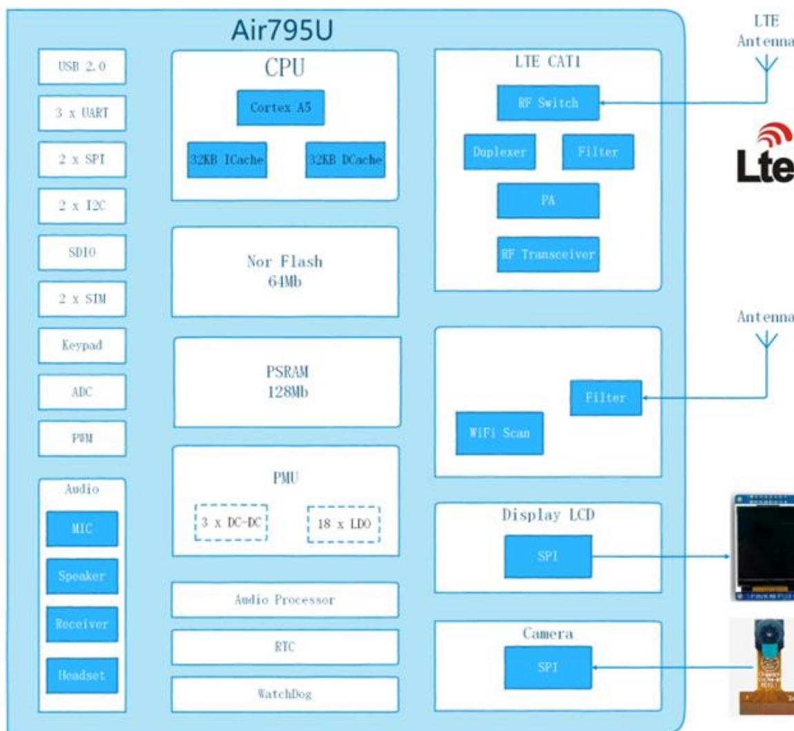
Chart1 : Functional Block Diagram
