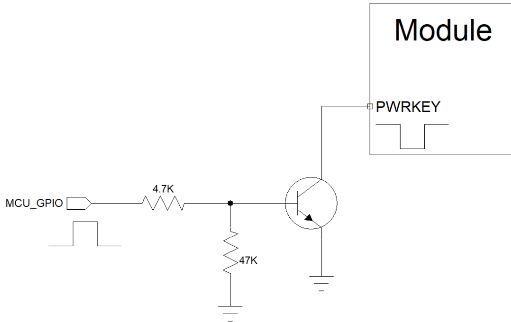
Chart5 : Open Set Driver Reference Power-Up Circuit
