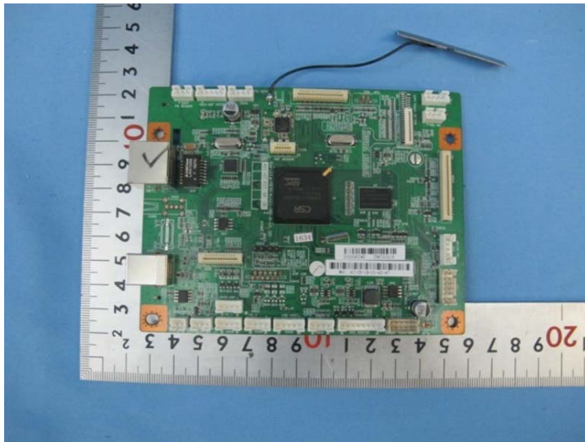
(Data Board Model: GORILLA-MFP(4IN1)-MB)
