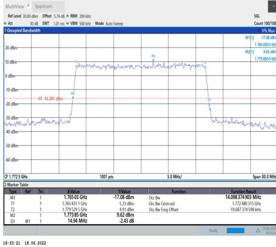
1-N66--15-15-H-9-CP-256QAM-Outer_Full-79@0-An t1-14.098-14.940-≤15-PASS
