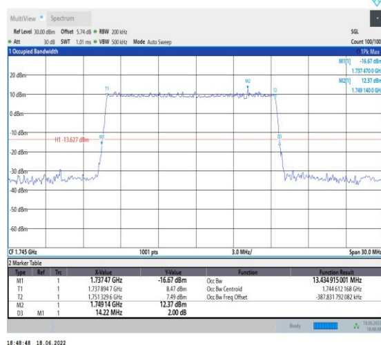
1-N66--15-15-M-5-DFT-256QAM-Outer_Full-75@0-A nt1-13.435-14.220-≤15-PASS
