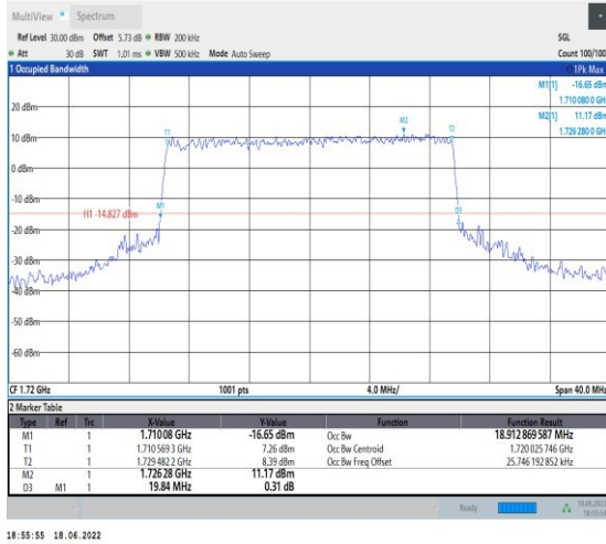
1-N66--15-20-L-8-CP-64QAM-Outer_Full-106@0-An t1-18.913-19.840-≤20-PASS
