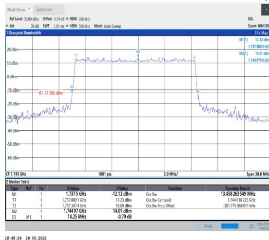
1-N66--15-15-M-3-DFT-16QAM-Outer_Full-75@0-An t1-13.458-14.250-≤15-PASS
