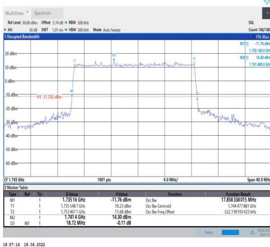
1-N66--15-20-M-1-DFT-QPSK-Outer_Full-100@0-An t1-17.858-18.720-≤20-PASS
