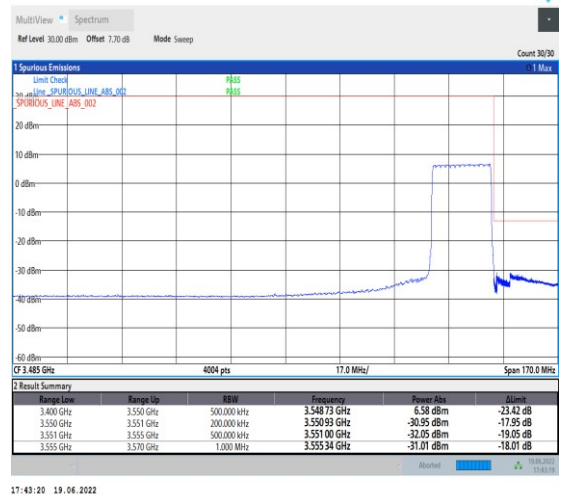
1-N78-3450-3550-PC2-30-20-H-6-CP-QPSK-Outer_Full-51@0-Ant1-PASS-see graph
