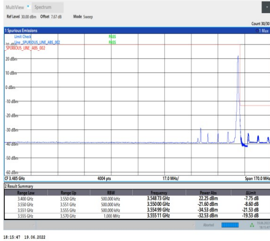
1-N78-3450-3550-PC2-30-50-H-2-DFT-PI2BPSK-Edge_1RB_Right-1@132-Ant1-PASS-see graph
