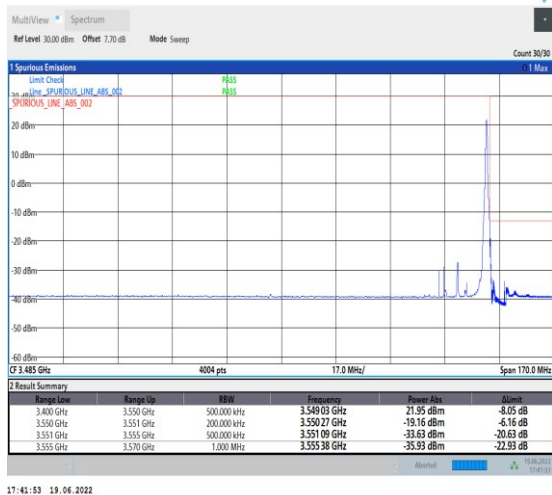
1-N78-3450-3550-PC2-30-20-H-5-CP-QPSK-Edge_1RB_Right-1@50-Ant1-PASS-see graph
