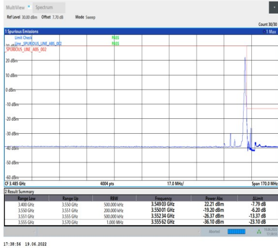
1-N78-3450-3550-PC2-30-20-H-2-DFT-PI2BPSK-Edge_1RB_Right-1@50-Ant1-PASS-see graph
