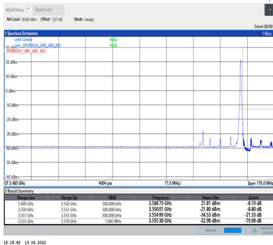
1-N78-3450-3550-PC2-30-50-H-5-CP-QPSK-Edge_1RB_Right-1@132-Ant1-PASS-see graph
