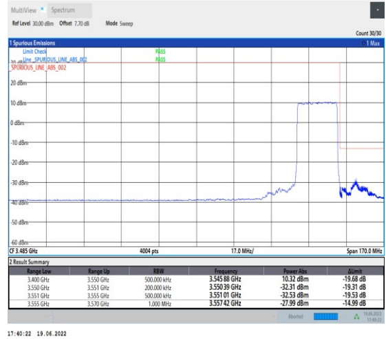
1-N78-3450-3550-PC2-30-20-H-3-DFT-PI2BPSK-Outer_Full-50@0-Ant1-PASS-see graph
