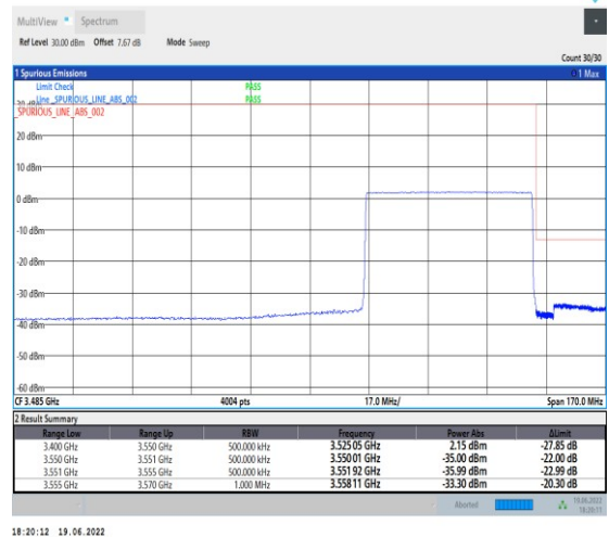
1-N78-3450-3550-PC2-30-50-H-6-CP-QPSK-Outer_Full-133@0-Ant1-PASS-see graph
