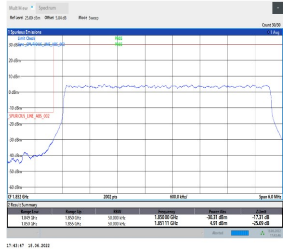
1-N25--15-5-L-3-DFT-PI2BPSK-Outer_Full-25@0-Ant1-seegraph-PASS-see graph
