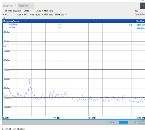
1-N25--15-40-M-1-DFT-PI2BPSK-Inner_1RB_Left-1 @1-0.009-0.15-Ant1--84.80--43-PASS
