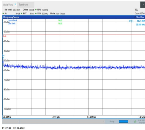
1-N25--15-40-M-1-DFT-PI2BPSK-Inner_1RB_Left-1 @1-30-1000-Ant1--48.21--23-PASS
