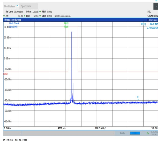
1-N25--15-40-H-1-DFT-PI2BPSK-Inner_1RB_Left-1 @1-1000-3000-Ant1--40.29--13-PASS
