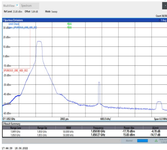
1-N25--15-5-L-4-CP-QPSK-Edge_1RB_Left-1@0-Ant1-seegraph-PASS-see graph
