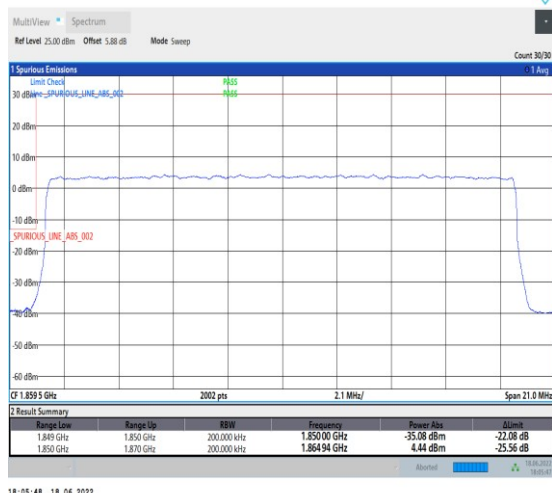
1-N25--15-20-L-3-DFT-PI2BPSK-Outer_Full-100@0-Ant1-seegraph-PASS-see graph
