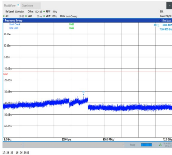
1-N25--15-40-L-1-DFT-PI2BPSK-Inner_1RB_Left-1 @1-3000-12000-Ant1--33.66--13-PASS
