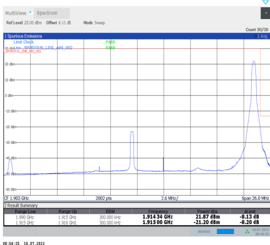
1-N25-PC3-15-25-H-5-CP-QPSK-Edge_1RB_Right-1@132-Ant1-seegraph-PASS-see graph
