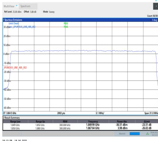
1-N25--15-30-L-3-DFT-PI2BPSK-Outer_Full-160@0-Ant1-seegraph-PASS-see graph
