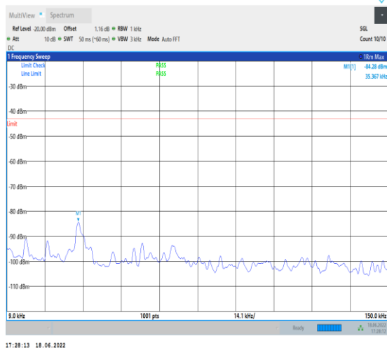
1-N25--15-40-H-1-DFT-PI2BPSK-Inner_1RB_Left-1 @1-0.009-0.15-Ant1--84.28--43-PASS
