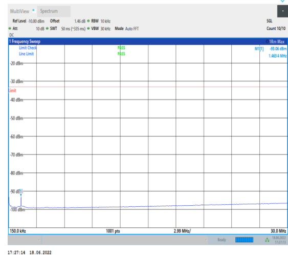
1-N25--15-40-M-1-DFT-PI2BPSK-Inner_1RB_Left-1 @1-0.15-30-Ant1--93.06--33-PASS
