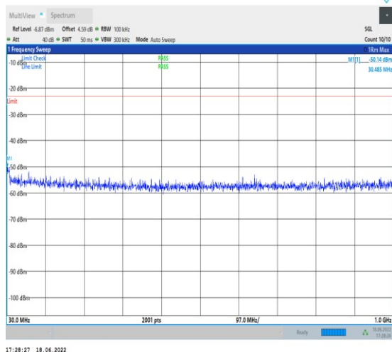
1-N25--15-40-H-1-DFT-PI2BPSK-Inner_1RB_Left-1 @1-30-1000-Ant1--50.14--23-PASS
