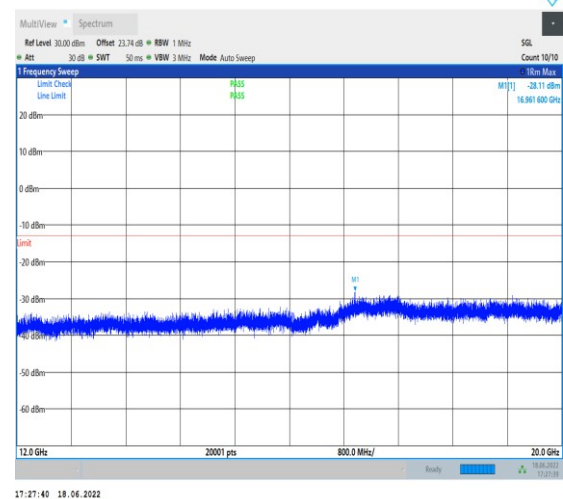
1-N25--15-40-M-1-DFT-PI2BPSK-Inner_1RB_Left-1 @1-12000-20000-Ant1--28.11--13-PASS
