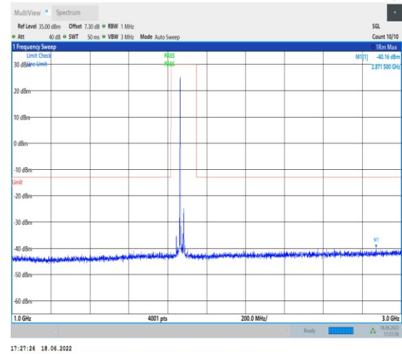
1-N25--15-40-M-1-DFT-PI2BPSK-Inner_1RB_Left-1 @1-1000-3000-Ant1--40.16--13-PASS
