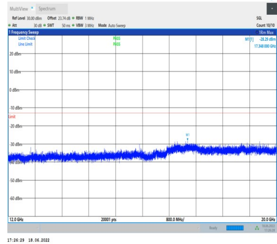
1-N25--15-40-L-1-DFT-PI2BPSK-Inner_1RB_Left-1@ 1-12000-20000-Ant1--28.29--13-PASS
