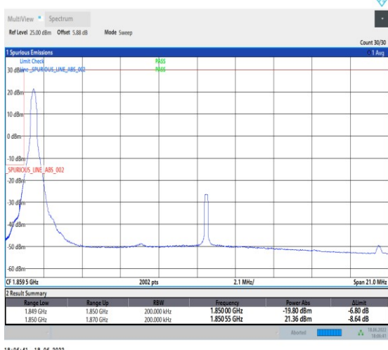
1-N25--15-20-L-4-CP-QPSK-Edge_1RB_Left-1@0-Ant1-seegraph-PASS-see graph
