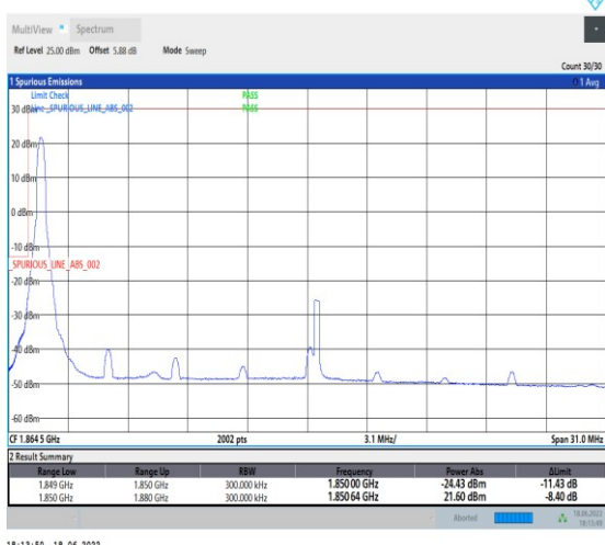
1-N25--15-30-L-4-CP-QPSK-Edge_1RB_Left-1@0-Ant1-seegraph-PASS-see graph
