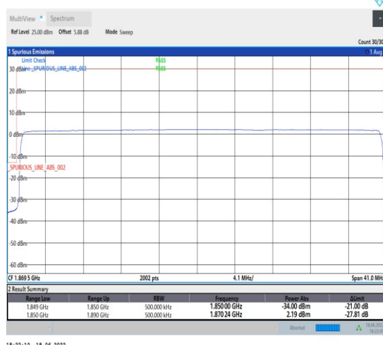
1-N25--15-40-L-6-CP-QPSK-Outer_Full-216@0-Ant1-seegraph-PASS-see graph
