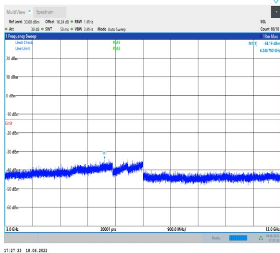
1-N25--15-40-M-1-DFT-PI2BPSK-Inner_1RB_Left-1 @1-3000-12000-Ant1--34.19--13-PASS
