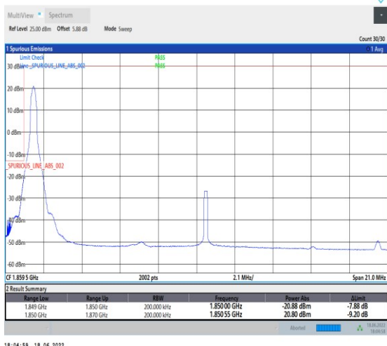
1-N25--15-20-L-1-DFT-PI2BPSK-Edge_1RB_Left-1@0-Ant1-seegraph-PASS-see graph
