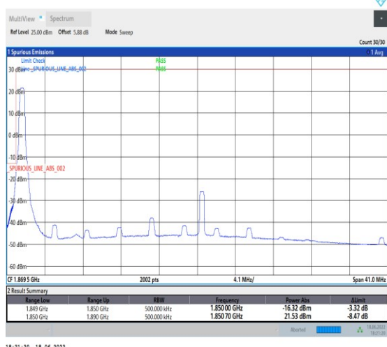
1-N25--15-40-L-4-CP-QPSK-Edge_1RB_Left-1@0-Ant1-seegraph-PASS-see graph
