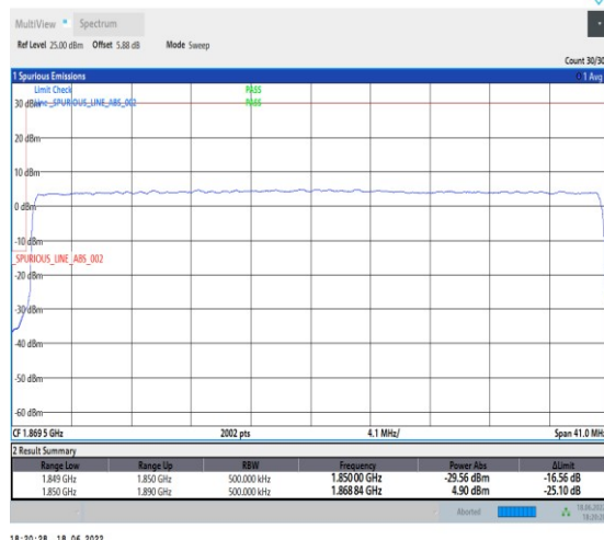
1-N25--15-40-L-3-DFT-PI2BPSK-Outer_Full-216@0-Ant1-seegraph-PASS-see graph
