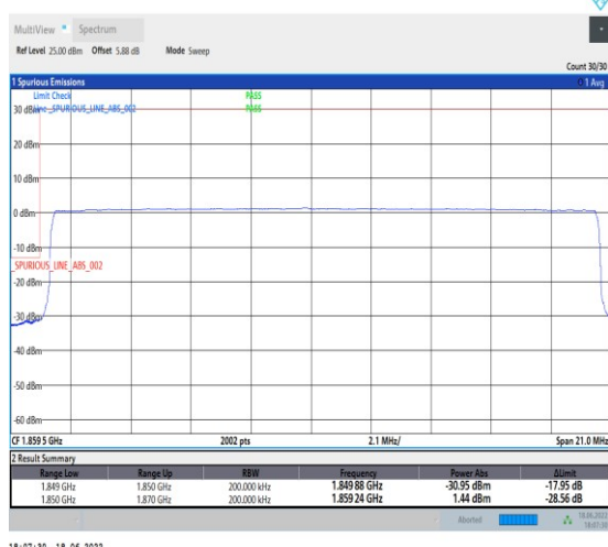
1-N25--15-20-L-6-CP-QPSK-Outer_Full-106@0-Ant1-seegraph-PASS-see graph
