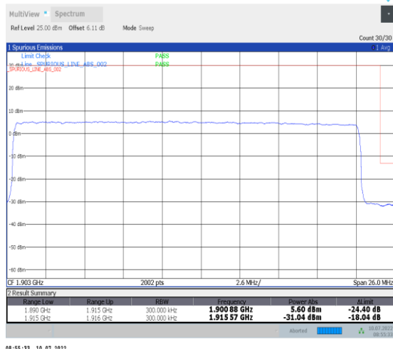
1-N25-PC3-15-25-H-3-DFT-PI2BPSK-Outer_Full-128@0-Ant1-seegraph-PASS-see graph
