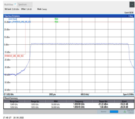
1-N25--15-5-L-6-CP-QPSK-Outer_Full-25@0-Ant1-seegraph-PASS-see graph
