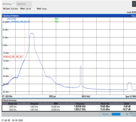
1-N25--15-5-L-1-DFT-PI2BPSK-Edge_1RB_Left-1@0-Ant1-seegraph-PASS-see graph
