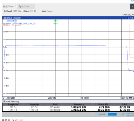
1-N25-PC3-15-25-H-6-CP-QPSK-Outer_Full-133@0-Ant1-seegraph-PASS-see graph
