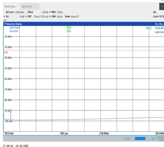
1-N25--15-40-H-1-DFT-PI2BPSK-Inner_1RB_Left-1 @1-0.15-30-Ant1--92.85--33-PASS
