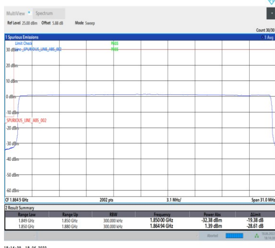
1-N25--15-30-L-6-CP-QPSK-Outer_Full-160@0-Ant1-seegraph-PASS-see graph
