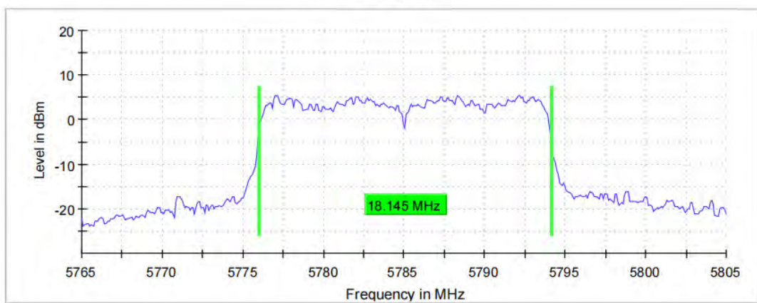
99 % Bandwidth
