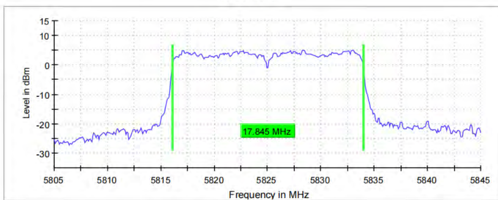
99 % Bandwidth
