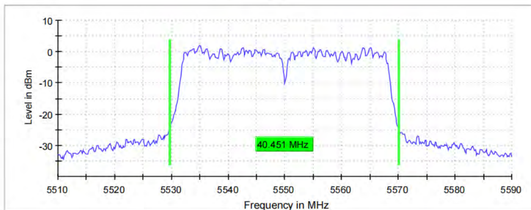
26 dB Bandwidth
