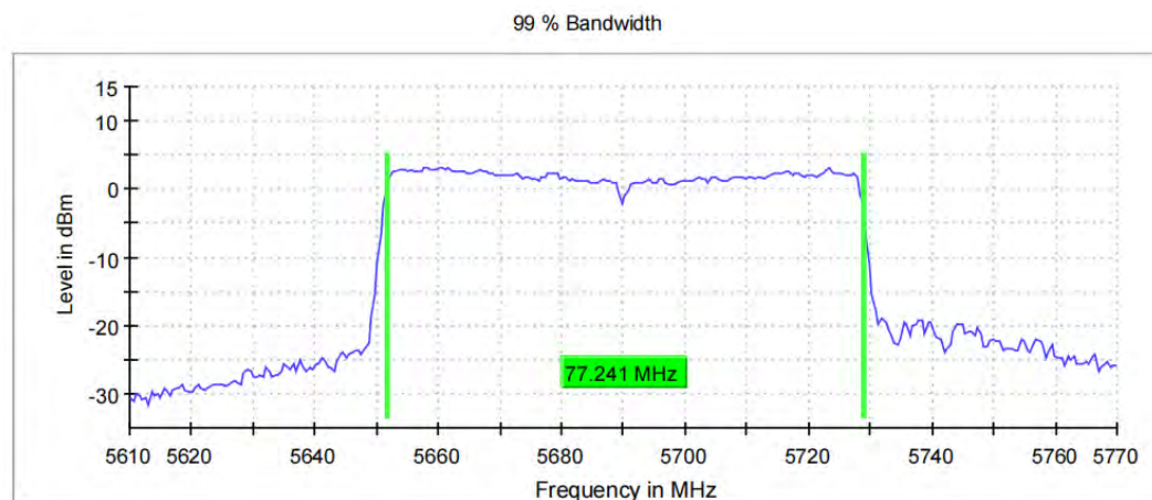
11AC80_Ant0_5690
