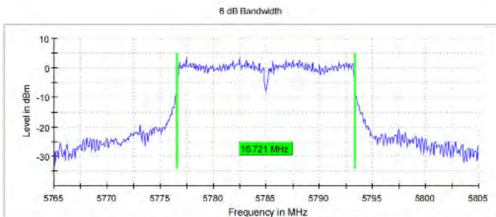
11A_Ant1_5785
