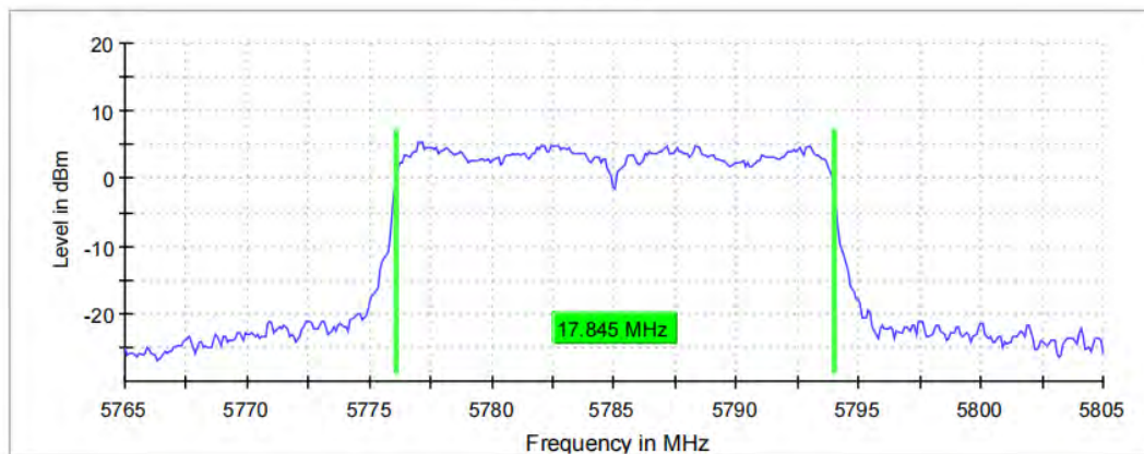
99 % Bandwidth
