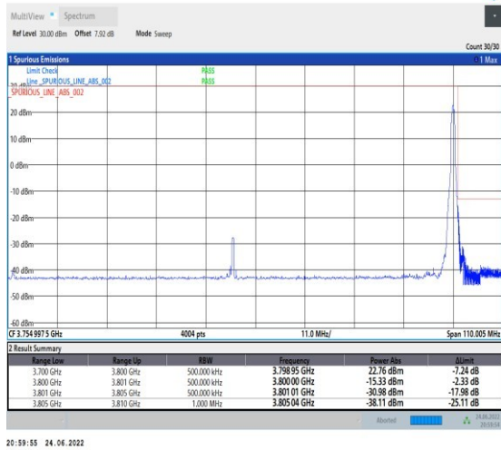
1-N78-3700-3800-PC2-30-100-H-2-DFT-PI2BPSK-Edge_1RB_Right-1@272-Ant1-PASS-see graph
