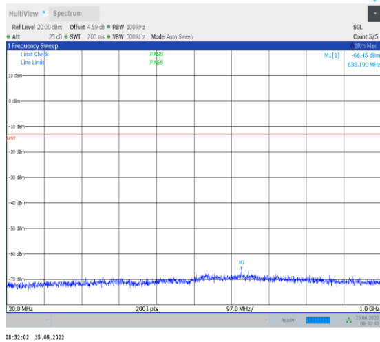
1-N78-3700-3800-PC2-30-100-L-1-DFT-PI2BPSK-In ner_1RB_Left-1@1-30-1000-Ant1--66.45--13-PASS
