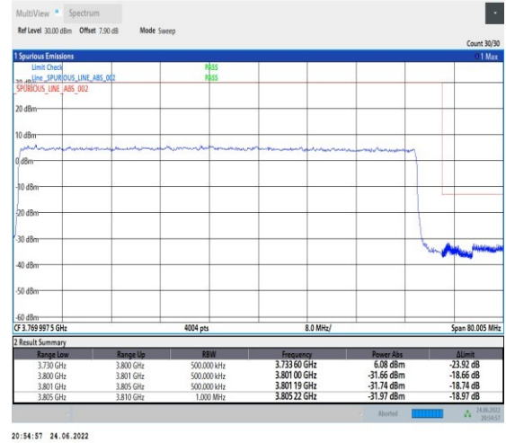
1-N78-3700-3800-PC2-30-70-H-3-DFT-PI2BPSK-Outer_Full-180@0-Ant1-PASS-see graph
