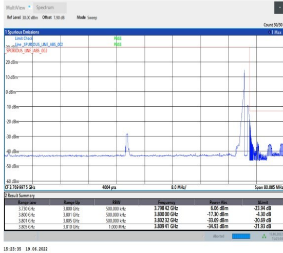
1-N78-3700-3800-PC2-30-70-H-2-DFT-PI2BPSK-Edge_1RB_Right-1@188-Ant1-PASS-see graph
