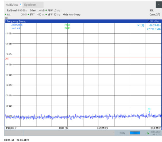
1-N78-3700-3800-PC2-30-100-L-1-DFT-PI2BPSK-In ner_1RB_Left-1@1-0.15-30-Ant1--86.33--33-PASS
