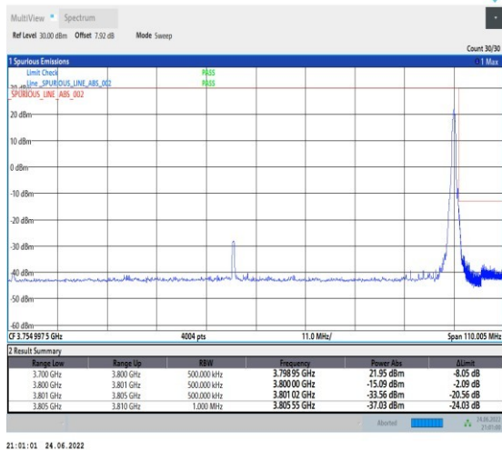
1-N78-3700-3800-PC2-30-100-H-5-CP-QPSK-Edge_1RB_Right-1@272-Ant1-PASS-see graph
