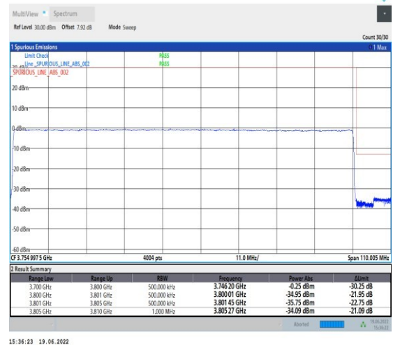
1-N78-3700-3800-PC2-30-100-H-6-CP-QPSK-Outer_Full-273@0-Ant1-PASS-see graph
