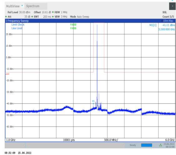
1-N78-3700-3800-PC2-30-100-L-1-DFT-PI2BPSK-In ner_1RB_Left-1@1-1000-6000-Ant1--41.11--13-PAS S
