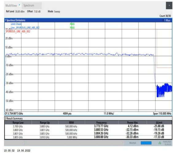
1-N78-3700-3800-PC2-30-100-H-3-DFT-PI2BPSK-Outer_Full-270@0-Ant1-PASS-see graph
