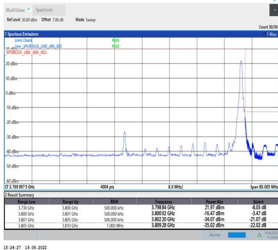
1-N78-3700-3800-PC2-30-70-H-5-CP-QPSK-Edge_1RB_Right-1@188-Ant1-PASS-see graph
