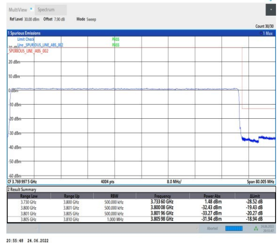
1-N78-3700-3800-PC2-30-70-H-6-CP-QPSK-Outer_Full-189@0-Ant1-PASS-see graph
