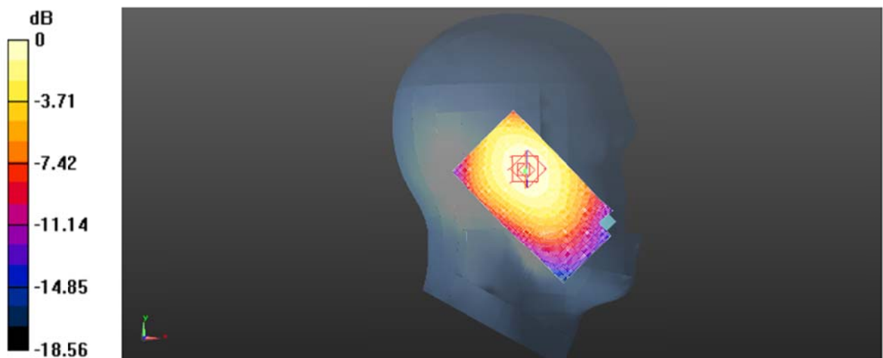
Left Head Cheek (WLAN middle Channel)
