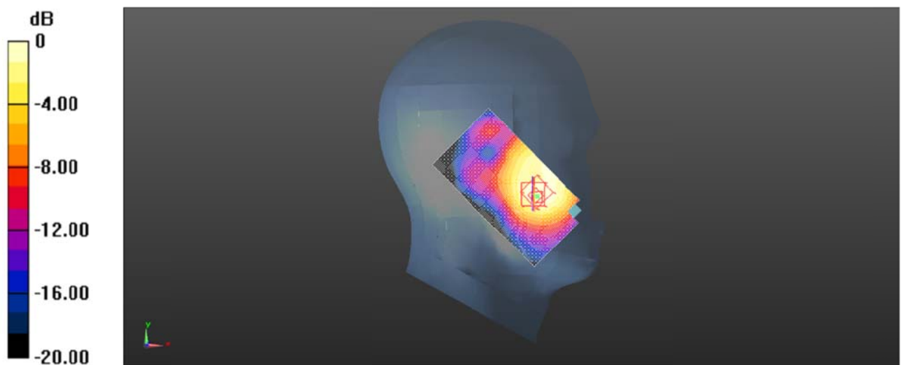
Left Head Tilt (DCS1800 Lowest Channel)
