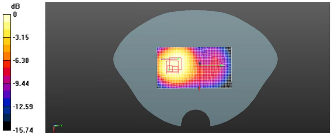
Body- worn Rear Side (WCDMA Band II Highest Channel)
