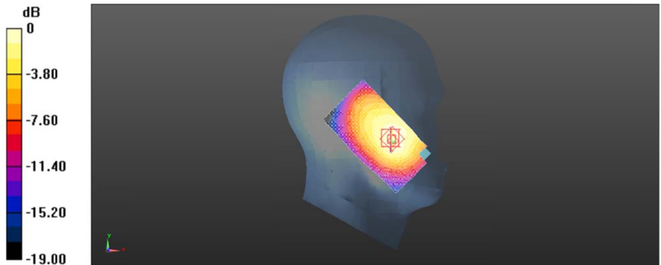
Left Head Cheek (WCDMA Band II Highest Channel)
