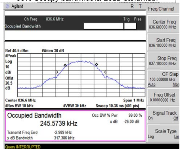
Channel 190
