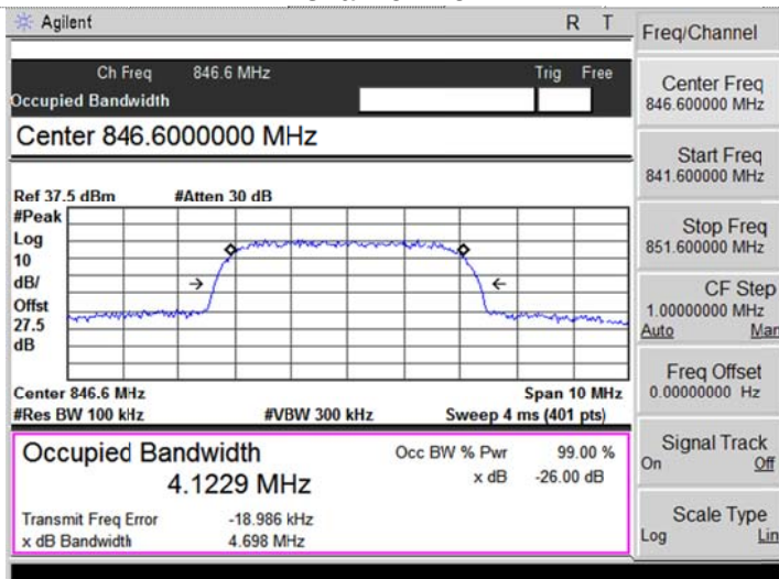
Channel 4233
