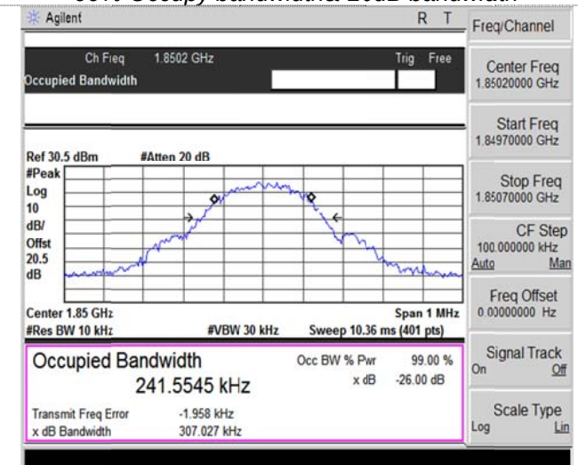
Channel 512
