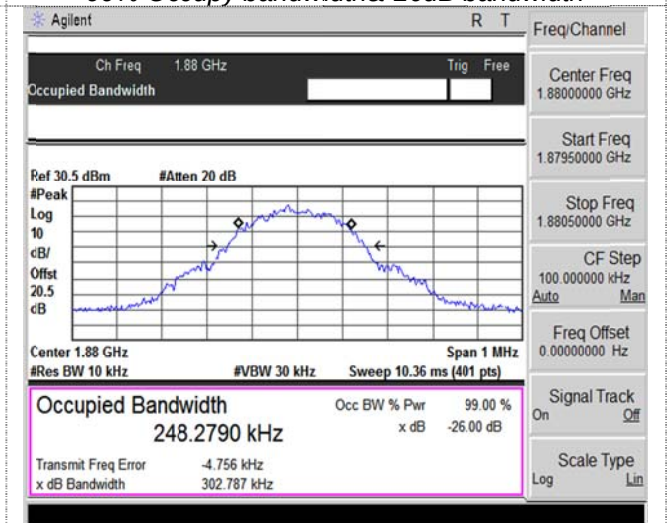
Channel 661
