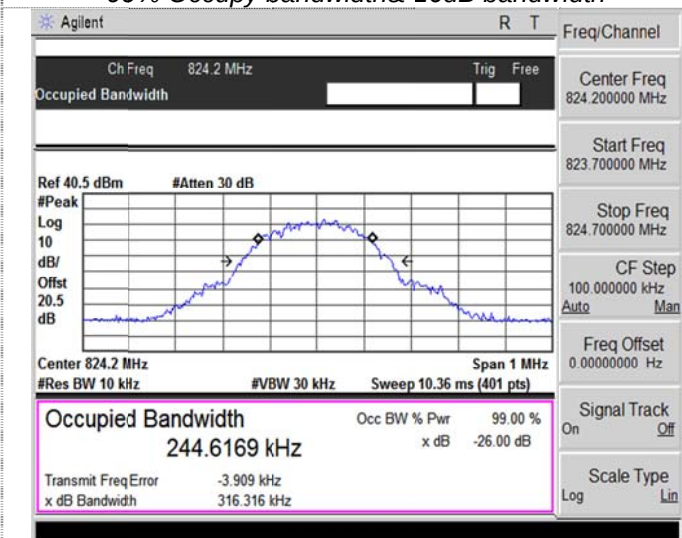
Channel 128
