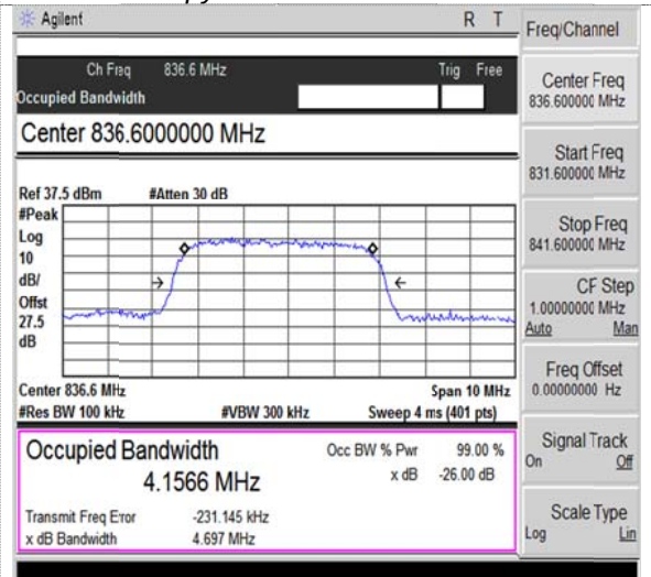
Channel 4183
