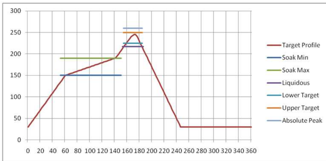
Figure 3: Recommended reflow temperature
