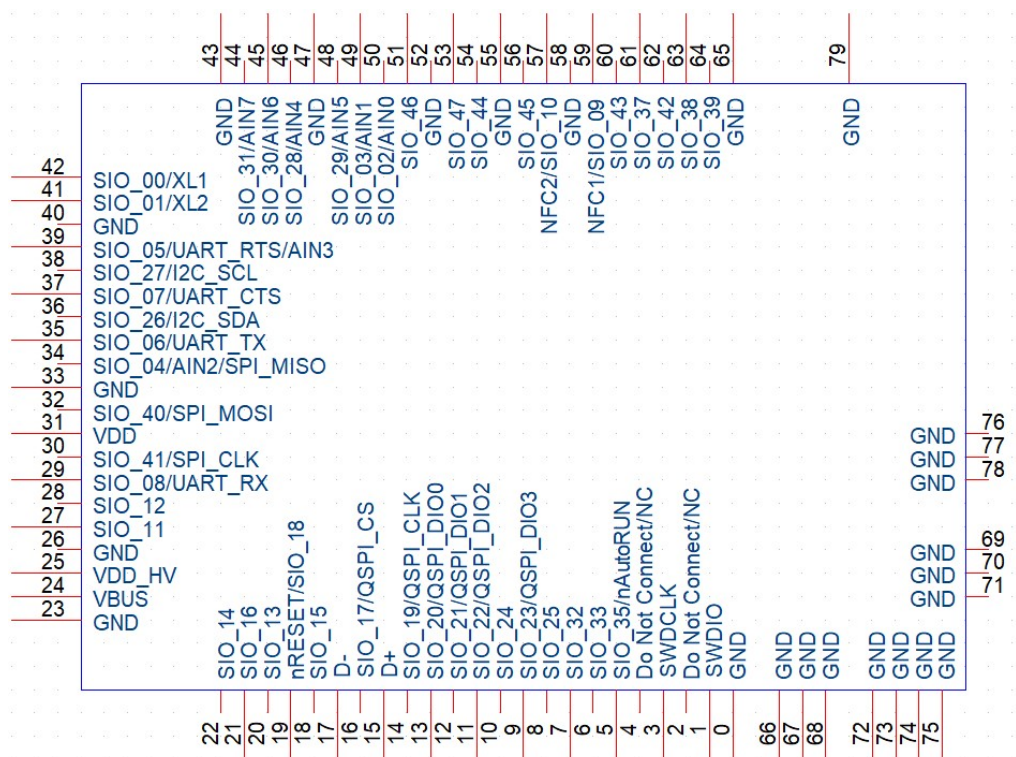
Figure 2: DSU840PA module pin-out (top view). Outer row pads (long red line) and inner row pads (short red line) shown.
