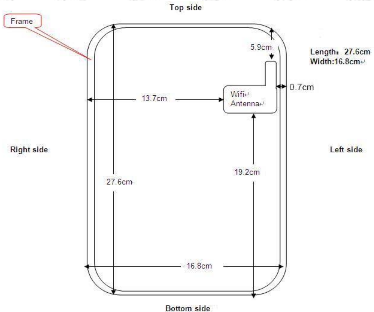
Figure2: The antenna position of the DUT
