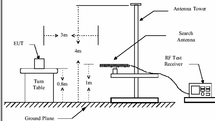
Above 1GHz
