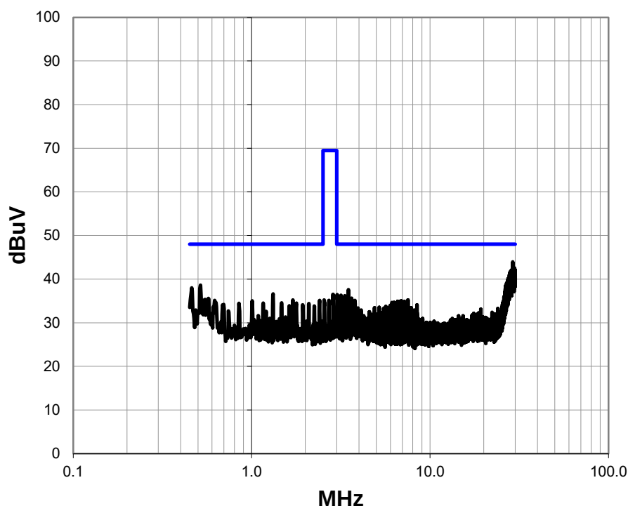
Peak Data - vs - Quasi Peak Limit
