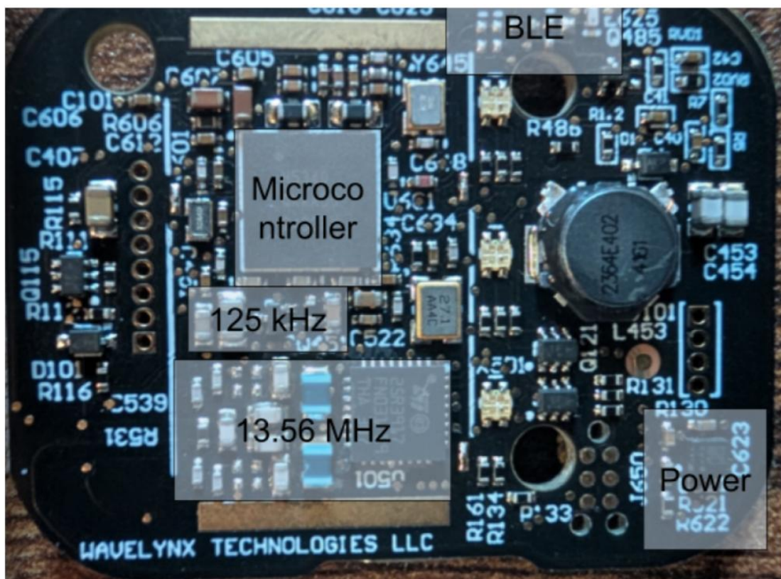
Main PCB top view
