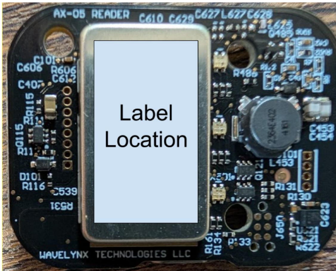
Main PCB with shield top view
