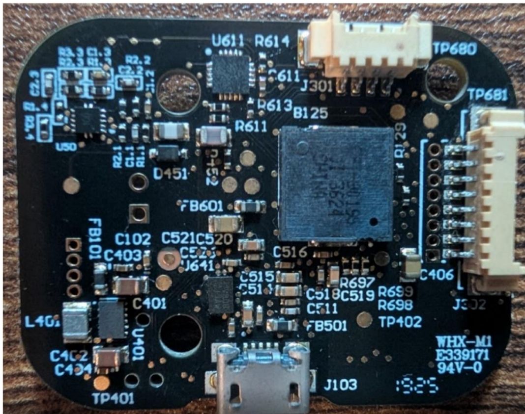
Main PCB bottom view
