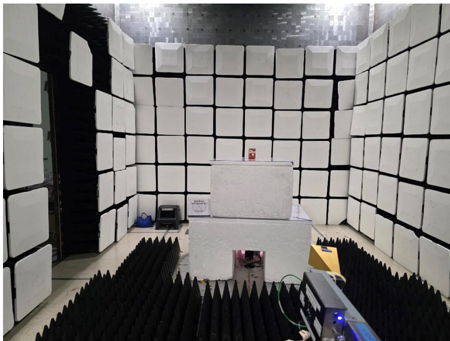
Figure 5 - Radiated emissions above 1 GHz (18 – 26.5 GHz), front view.
