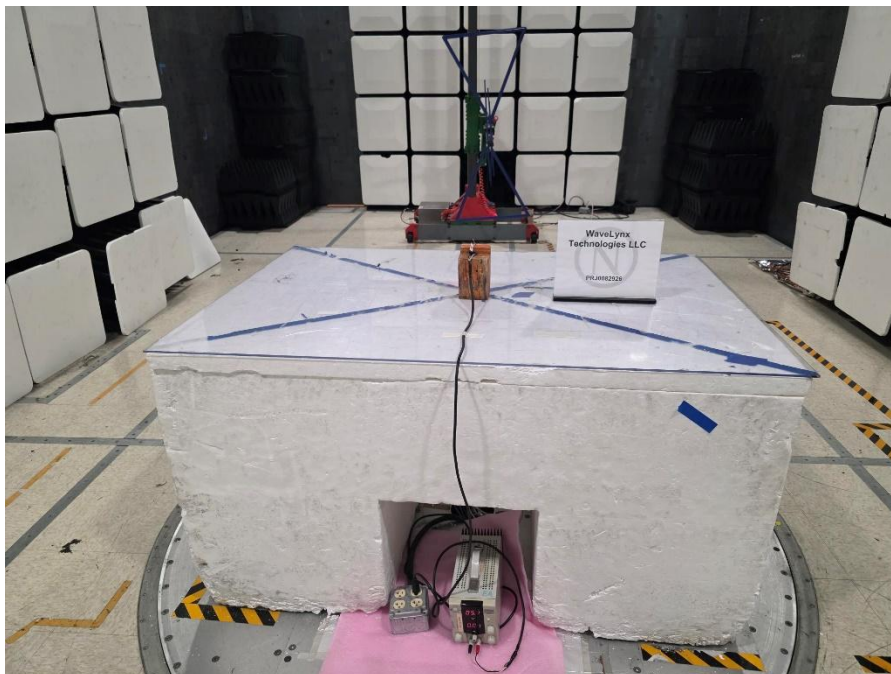
Figure 6 - Radiated emissions below 1 GHz (30 – 150 MHz), rear view.
