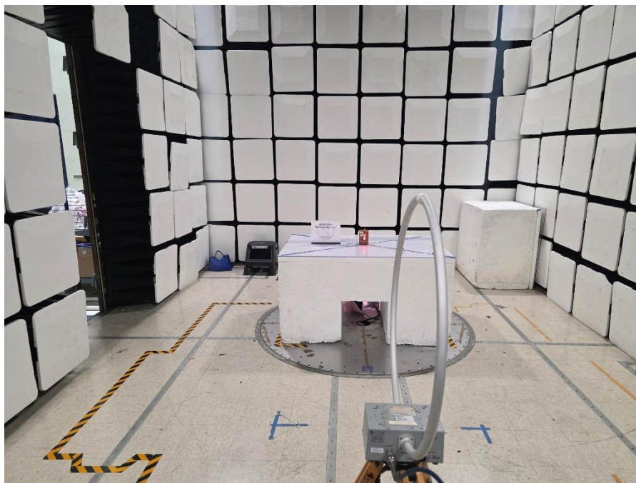
Figure 3 - Radiated emissions below 30 MHz, 90 Degrees, front view
