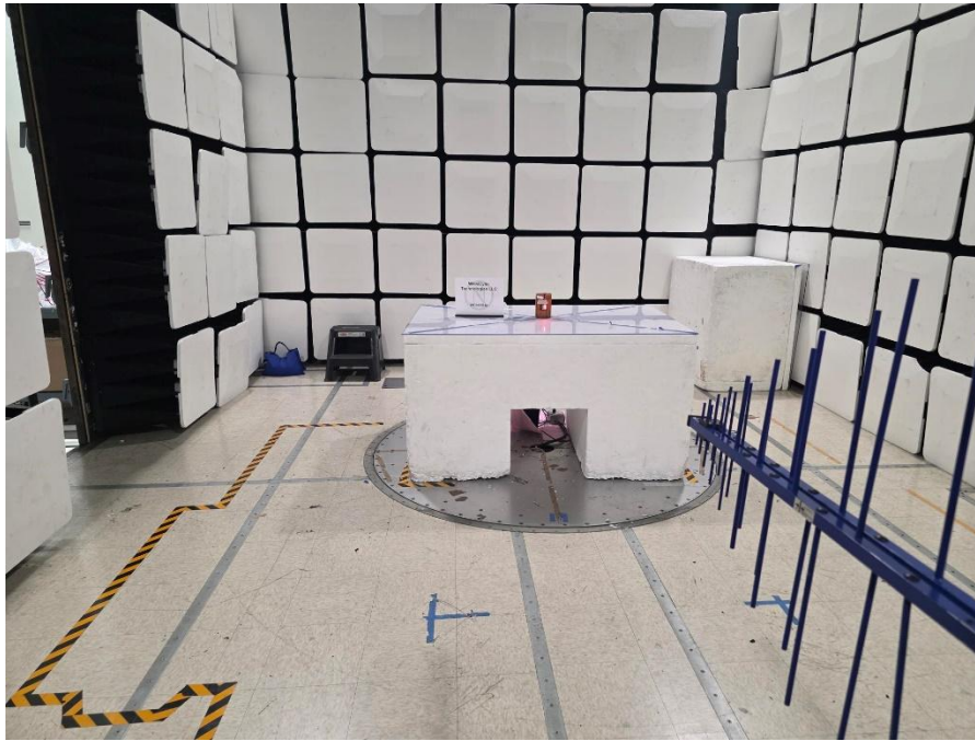
Figure 5 - Radiated emissions below 1 GHz, front view.
