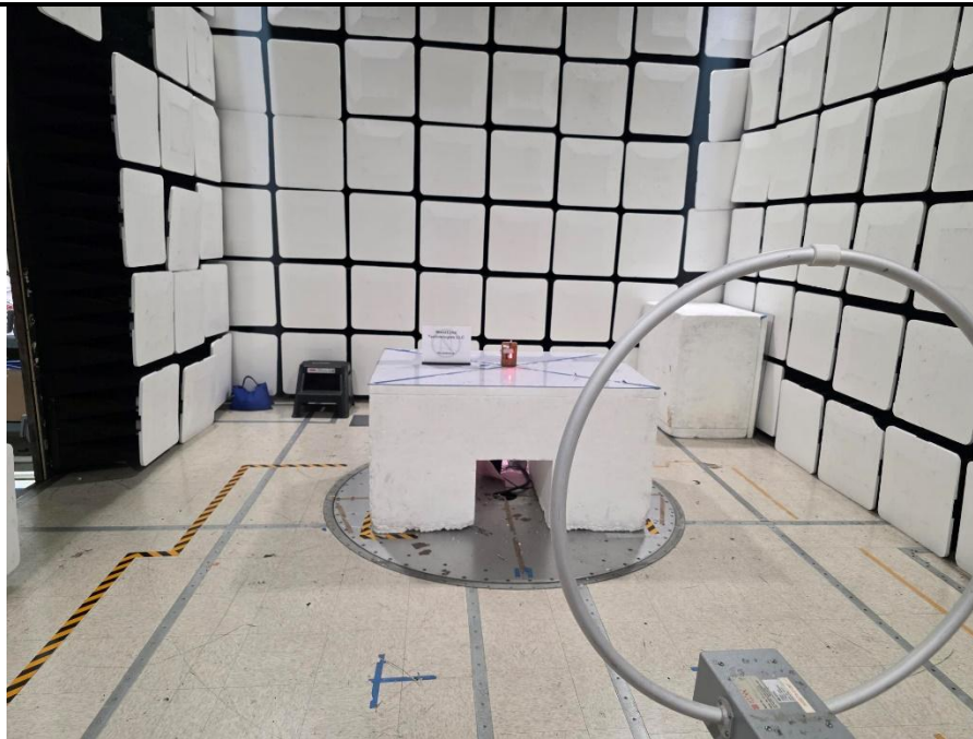
Figure 1 - Radiated emissions below 30 MHz, 0 Degree, front view
