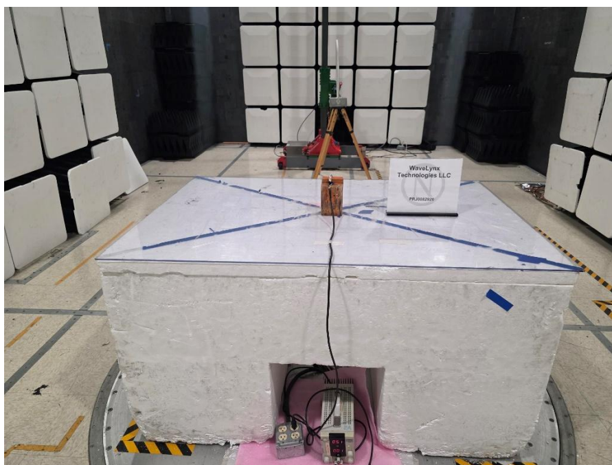
Figure 4 - Radiated emissions below 30 MHz, 90 Degrees, rear view
