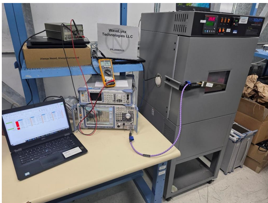
Figure 9 – Test setup, frequency stability – Varying Voltage
