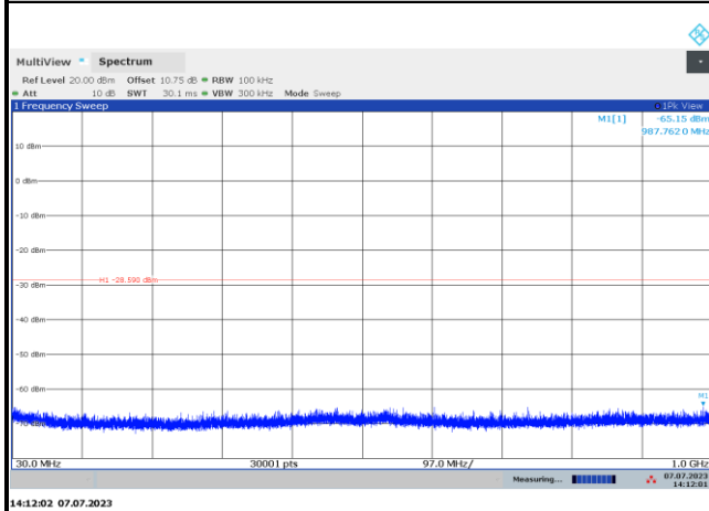
Conducted Spurious Emission Plot on Bluetooth LE 2Mbps GFSK Channel 19
