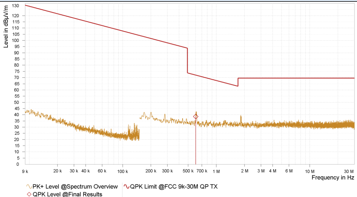
Radiated Spurious Emission 9 kHz – 30 MHz (Antenna Position 180°): 2.4GHz ISM Mid
