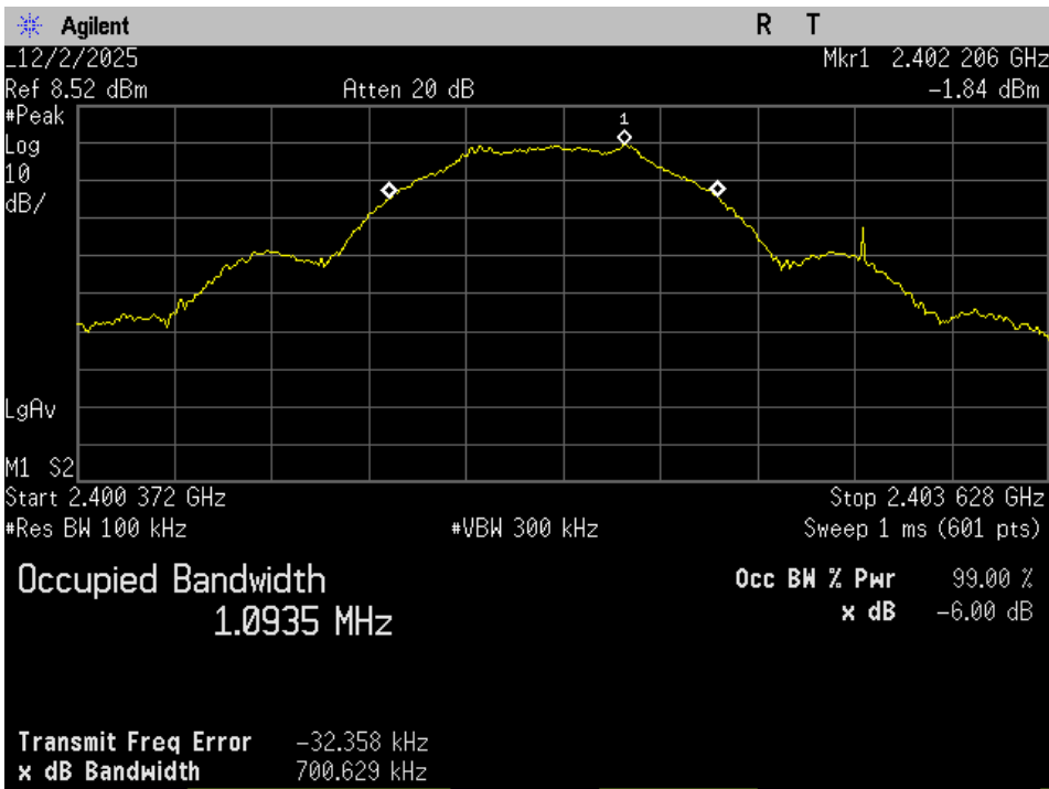
BLE 1M, Low Channel, 2402 MHz, 6dB OBW
