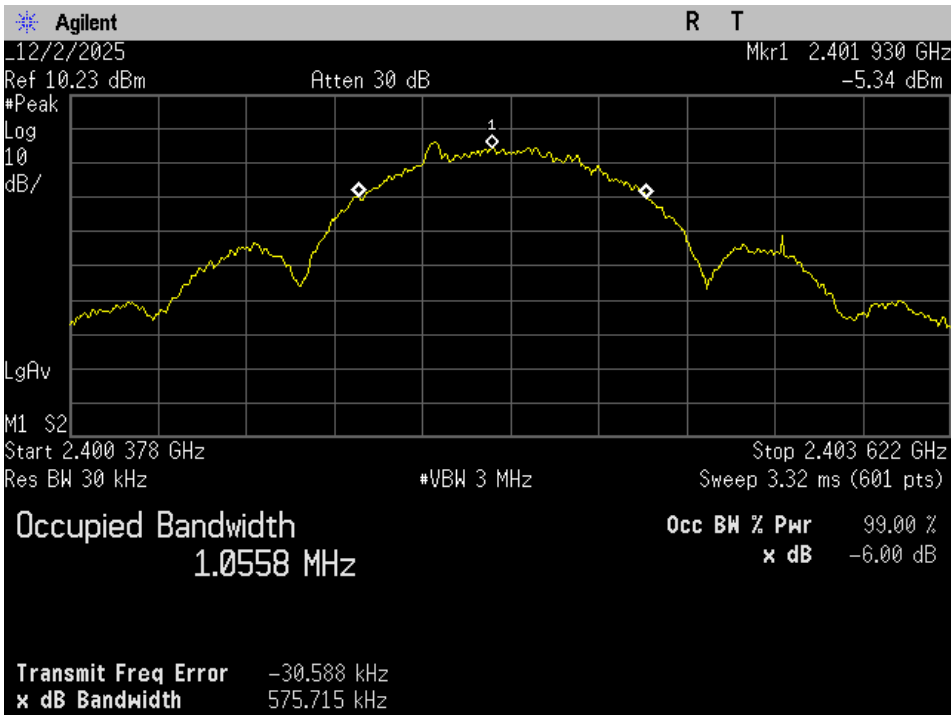
BLE 1M, Low Channel, 2402 MHz, 99% OBW
