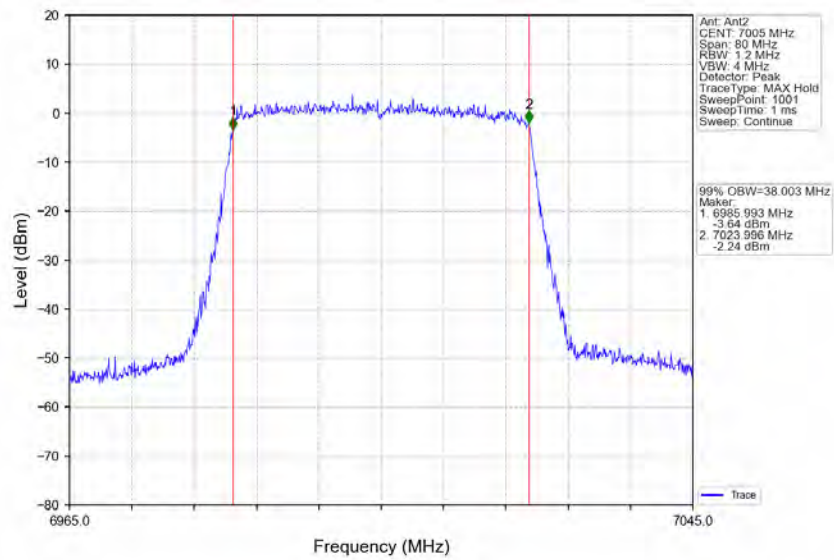
802.11ax(HEW40)_MCH_7005MHz_RU484_Left_Ant2_NTNV
