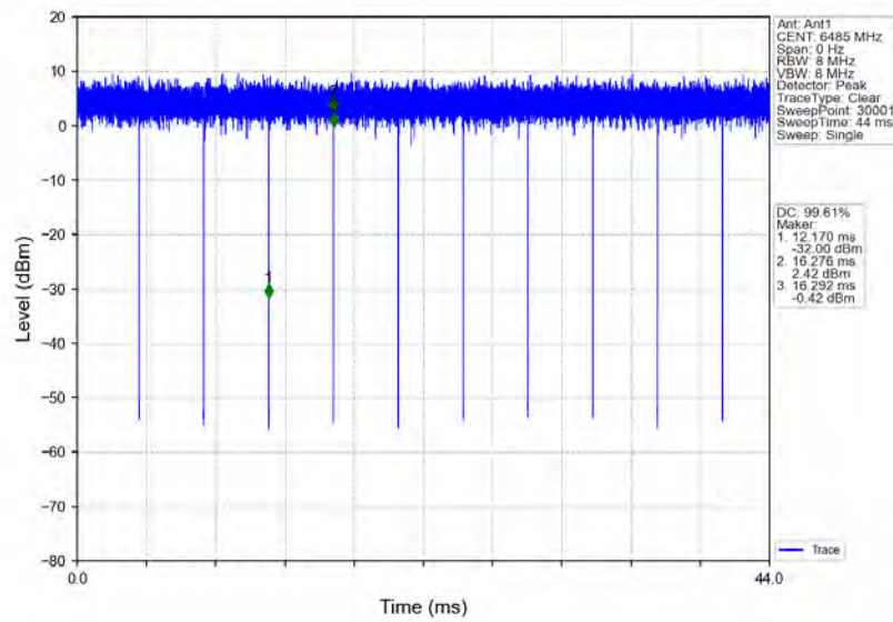
802.11ax(HEW40)_MCH_6485MHz_RU484_Left_Ant1_NTNV
