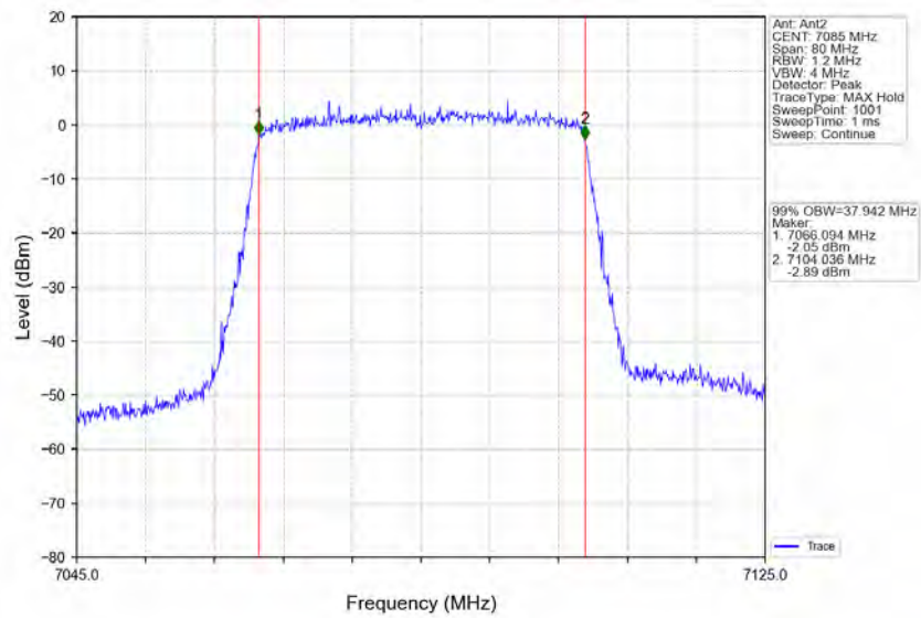
802.11ax(HEW40)_HCH_7085MHz_RU484_Left_Ant2_NTNV
