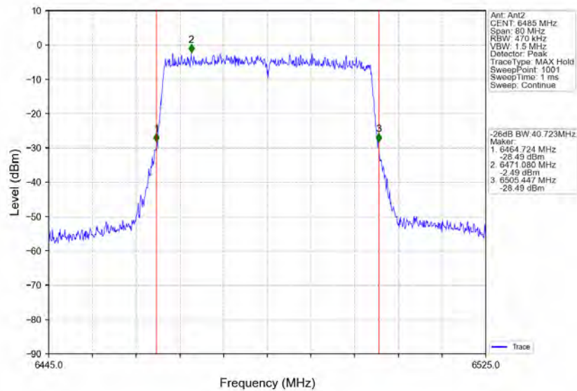
802.11ax(HEW40)_MCH_6485MHz_RU484_Left_Ant2_NTNV
