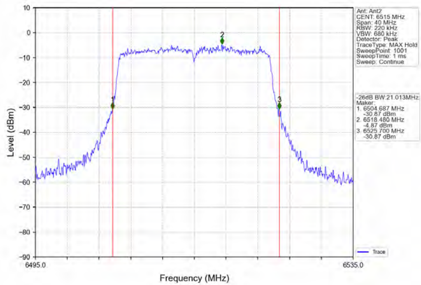
802.11ax(HEW20)_HCH_6515MHz_RU242_Left_Ant2_NTNV
