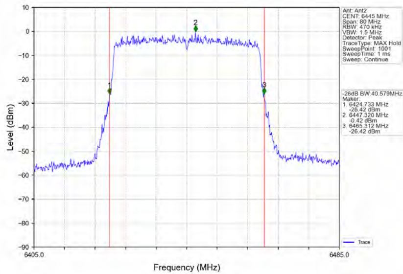
802.11ax(HEW40)_LCH_6445MHz_RU484_Left_Ant2_NTNV
