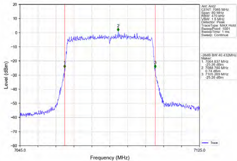
802.11ax(HEW40)_HCH_7085MHz_RU484_Left_Ant2_NTNV
