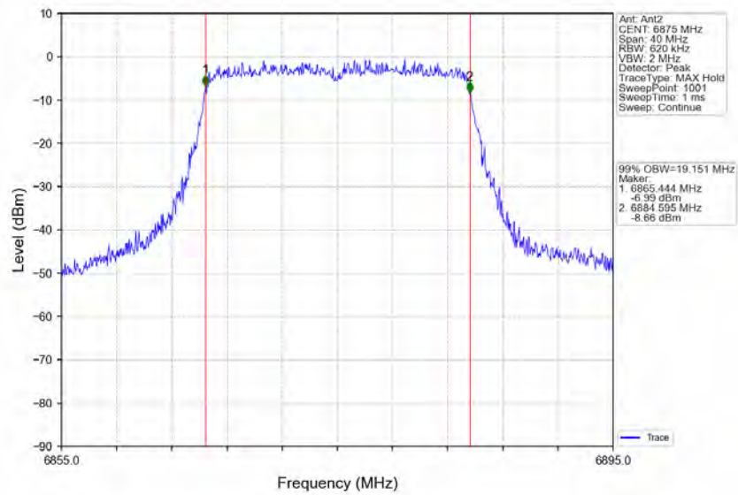
802.11ax(HEW20)_HCH_6875MHz_RU242_Left_Ant2_NTNV
