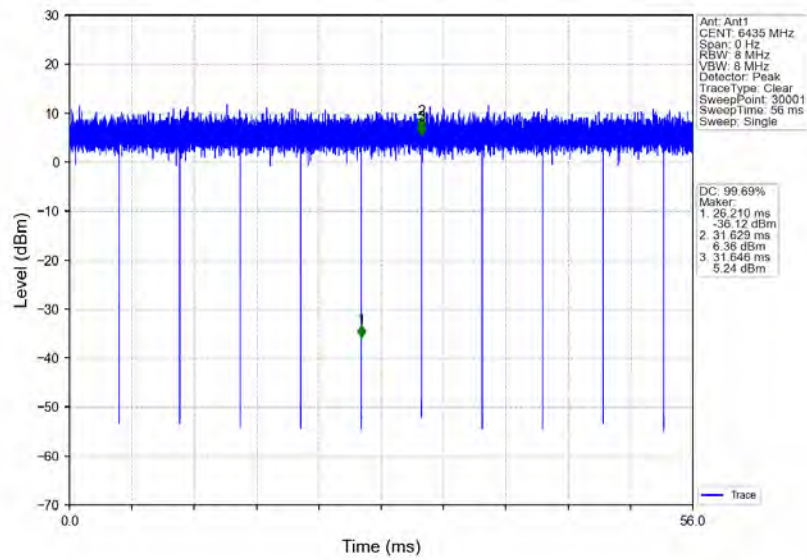
802.11ax(HEW20)_LCH_6435MHz_RU242_Left_Ant1_NTNV
