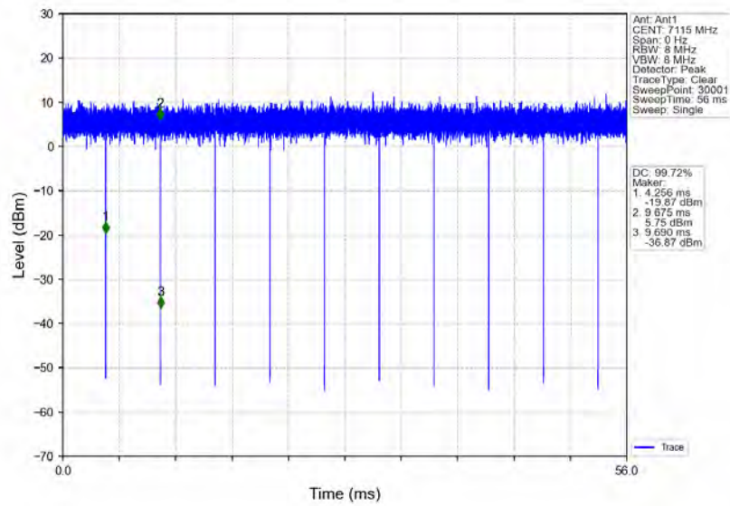
802.11ax(HEW20)_HCH_7115MHz_RU242_Left_Ant1_NTNV
