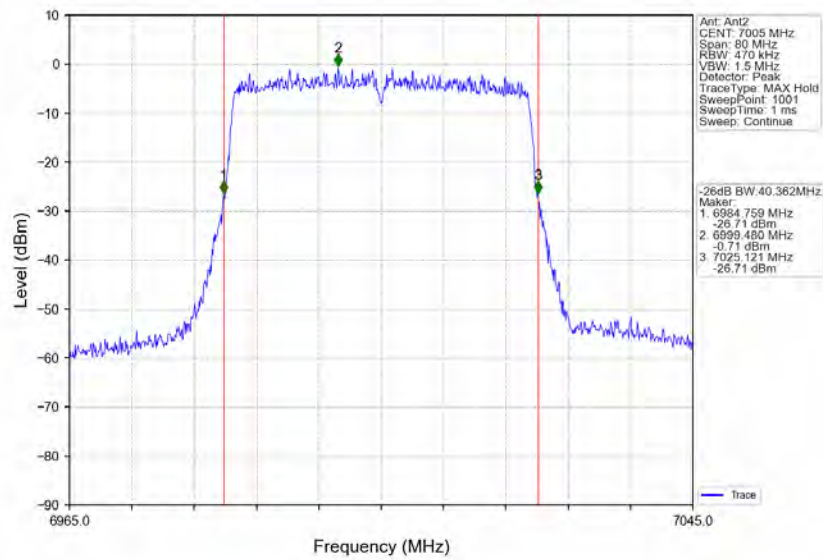
802.11ax(HEW40)_MCH_7005MHz_RU484_Left_Ant2_NTNV
