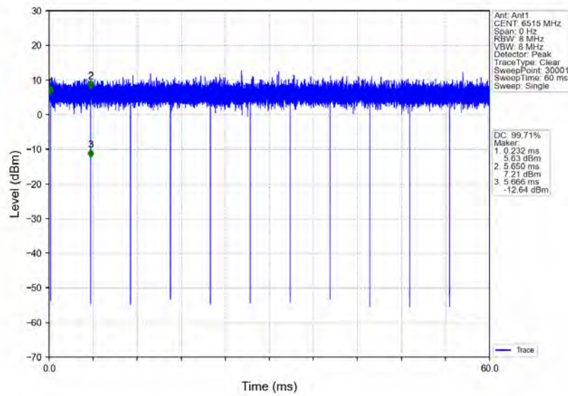
802.11ax(HEW20)_HCH_6515MHz_RU242_Left_Ant1_NTNV
