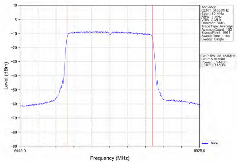
802.11ax(HEW40)_MCH_6485MHz_RU484_Left_Ant2_NTNV
