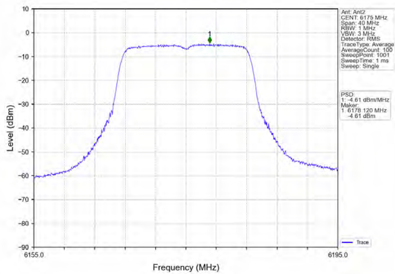
802.11a_MCH_6175MHz_Ant2_NTNV
