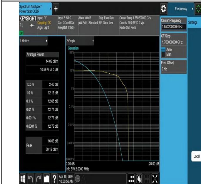
EGPRS1900-512-2-PASS
