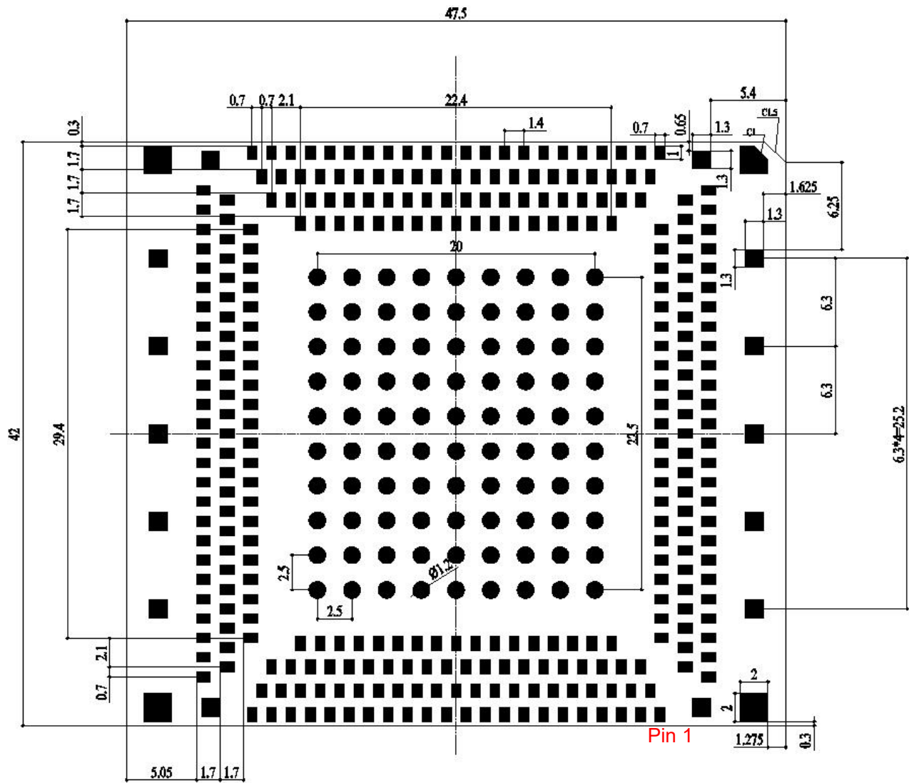
Figure 42: Module Bottom Dimensions (Unit: mm)
