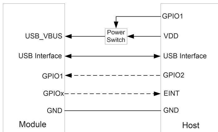
Figure 3: Low Power Mode Application Without Suspend Function
