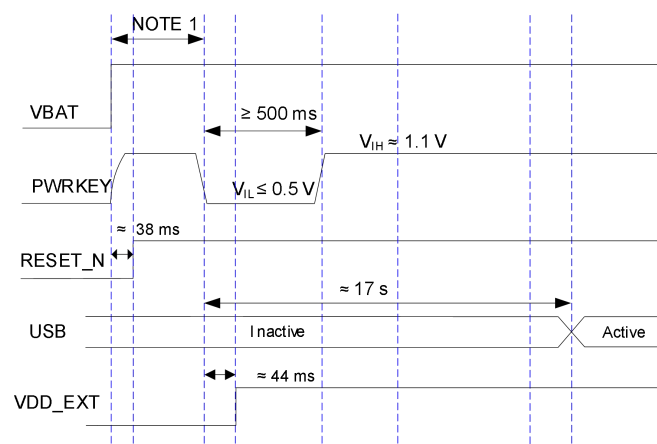
Figure 10: Power-up Timing
