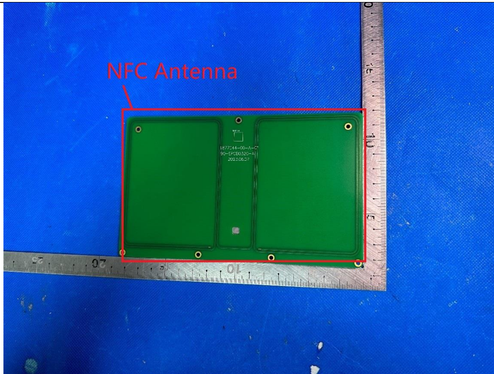
(1) EUT Photo – NFC Antenna
