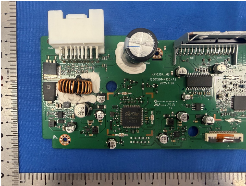
Photo 9: Internal View for BLE Chip
