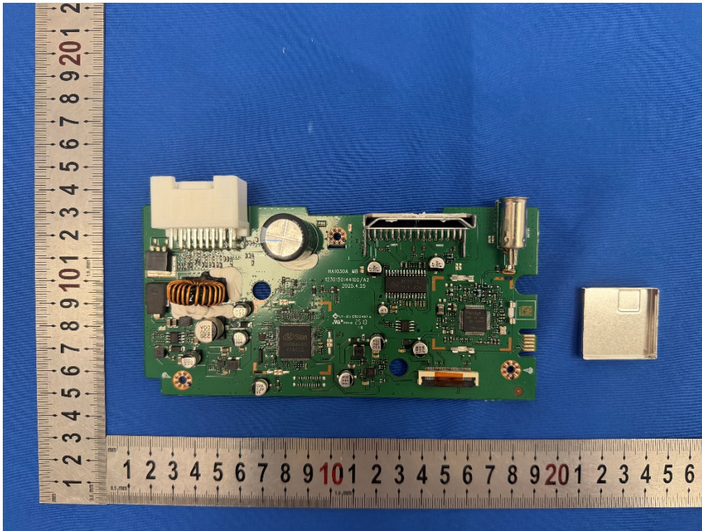
Photo 7: Internal View for LTE chip
