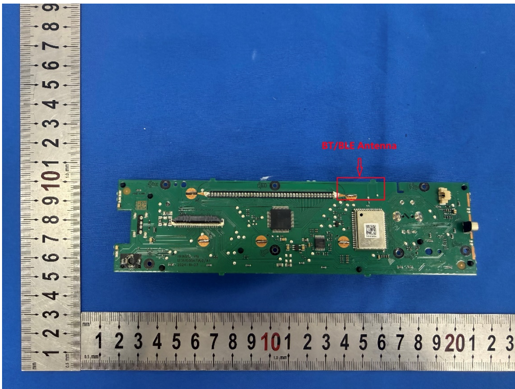
Photo 12: Internal View for BT/BLE Antenna
