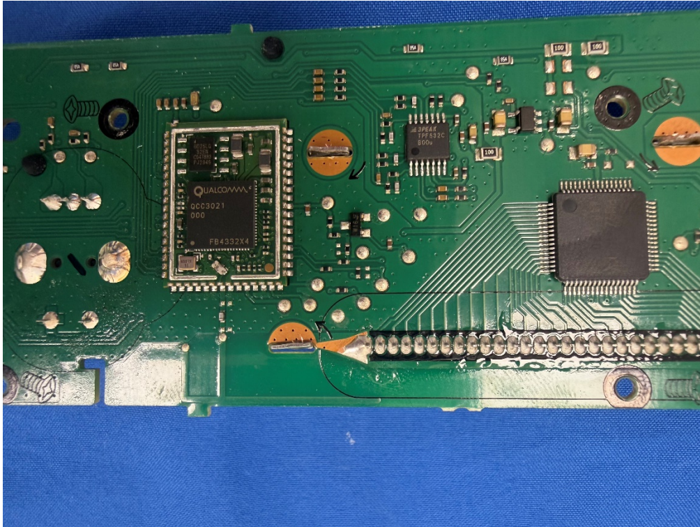
Photo 18: Internal View for PCB
