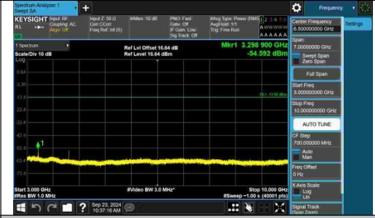
Band5-1.4MHz-16QAM-20407-6RB#0-3000 ~10000-PASS
