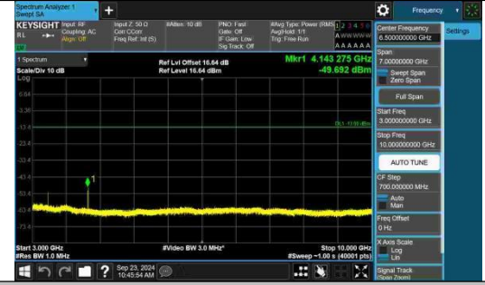
Band5-5MHz-QPSK-20425-1RB#24-3000~10000-PASS
