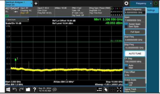
Band5-3MHz-QPSK-20415-1RB#14-3000~10000-PASS
