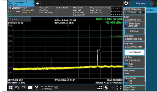
Band5-1.4MHz-16QAM-20643-6RB#0-1000 ~3000-PASS
