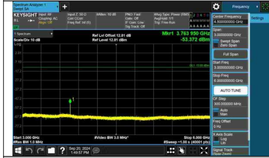
Band2-5MHz-QPSK-18900-1RB#24-3000~6 000-PASS
