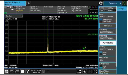
Band2-5MHz-16QAM-18900-1RB#0-1000~3 000-PASS
