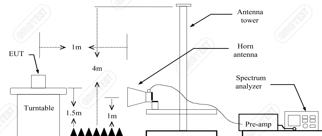
Figure 4. Above 18GHz radiated emissions test configuration
